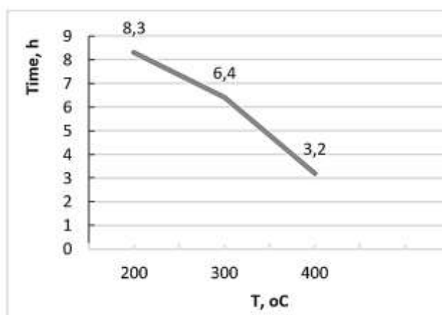
Figure 6. Dependence of the operating time on the temperature in the center of the furnace
