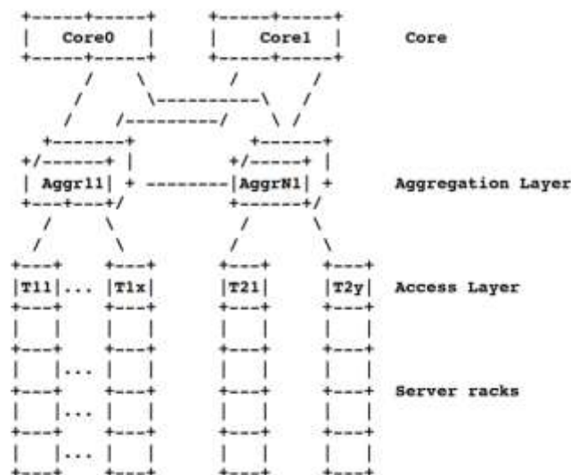
Figure 2. A Generalized 3 Layer Data Center Network Architecture
