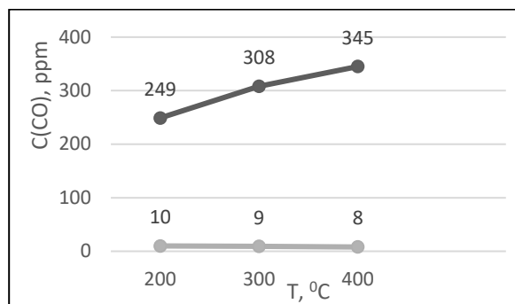
Figure 4. The dependence of CO content on furnace temperature
