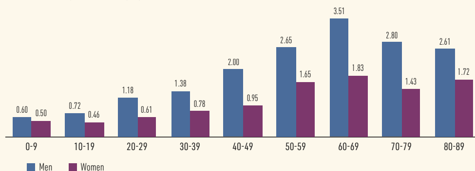
Geometric mean of mercury in hair, by age group, in \mu\text{g/g} Random sample in total population of the Faroe Islands 2020
