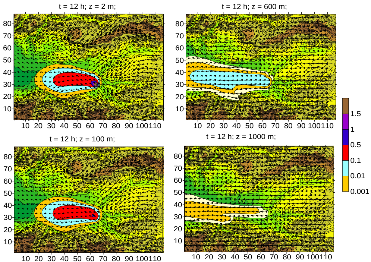
Fig. 1. Wind velocity and dust concentration distribution at the height of z = 2, 100, 600 and 1000 meters from the earth surface in case of background eastern quiet wind, t = 12 \text{ h} .
