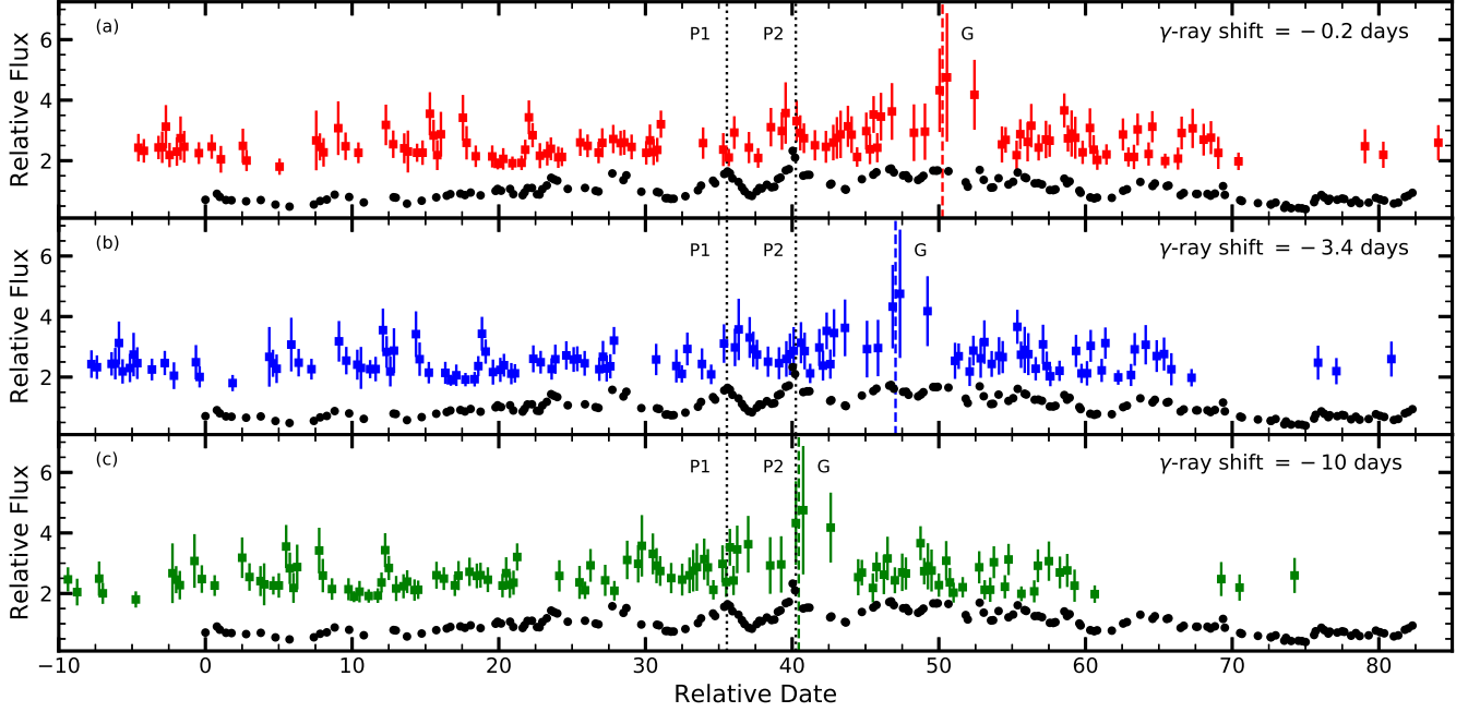
Figure 24. WEBA R -band (black circles) and Fermi \gamma -ray (colored squares) light curves. See text for scaling. The \gamma -ray light curve is shifted by the indicated amount along the x -axis in each panel, and upper limits are omitted for clarity. The optical peaks P1 and P2 have been identified with dotted black lines, and \gamma -ray peak G with dashed colored lines.
