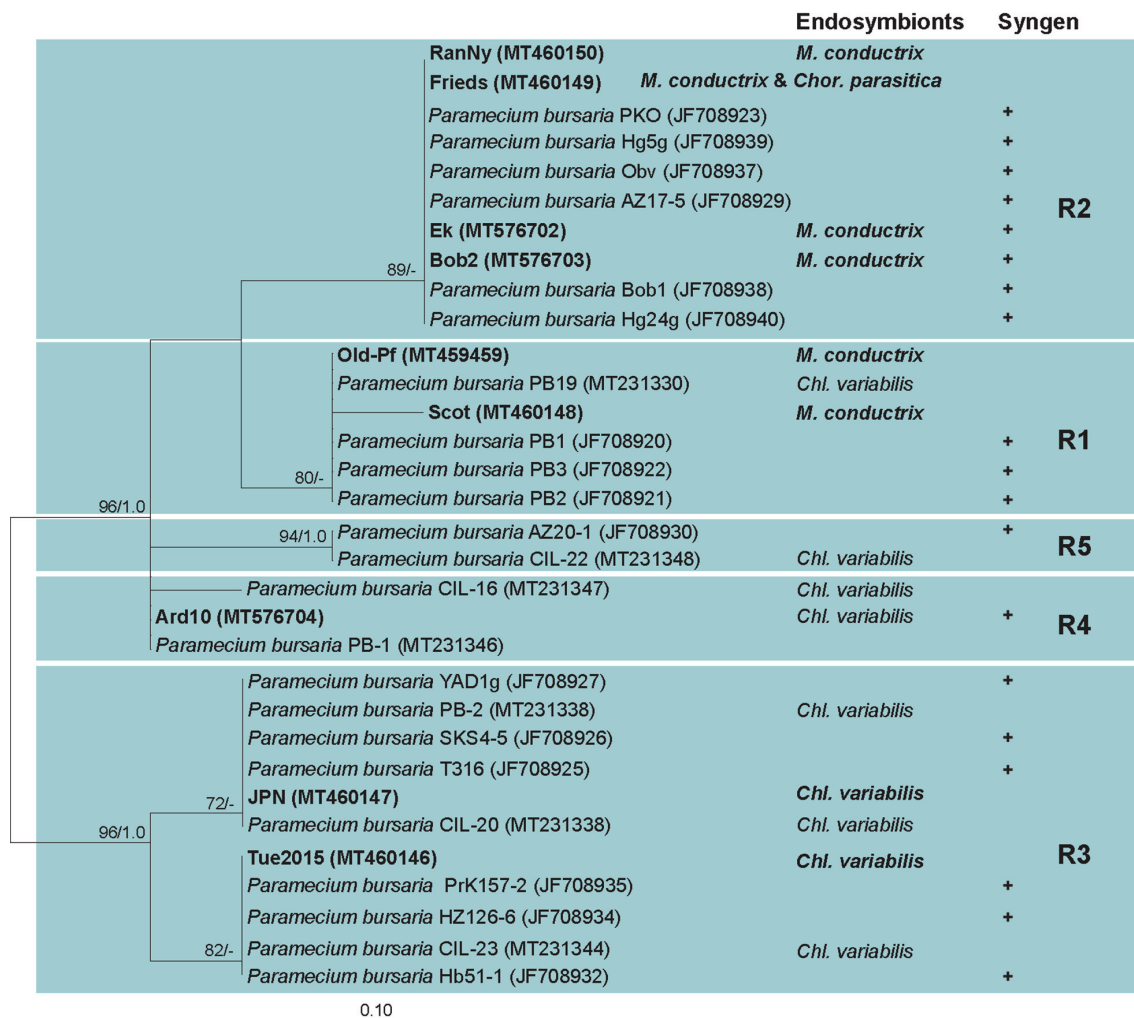
Figure 4. Syngen affiliation of Paramecium bursaria strains based on the internal transcribed spacer (ITS) region spanning ITS1-5.8S-ITS2. Unrooted Maximum likelihood tree based on 506 aligned positions is shown. GTR+I was used as evolutionary model. Bootstrap values above 70 % and Bayesian Inference values above 0.95 are indicated. The five syngens are highlighted as R1 to R5, a plus marks a strain whose mating behaviour was previously experimentally determined. The identity of the algal symbiont if known is provided. Sequences marked in bold were obtained in this study.
