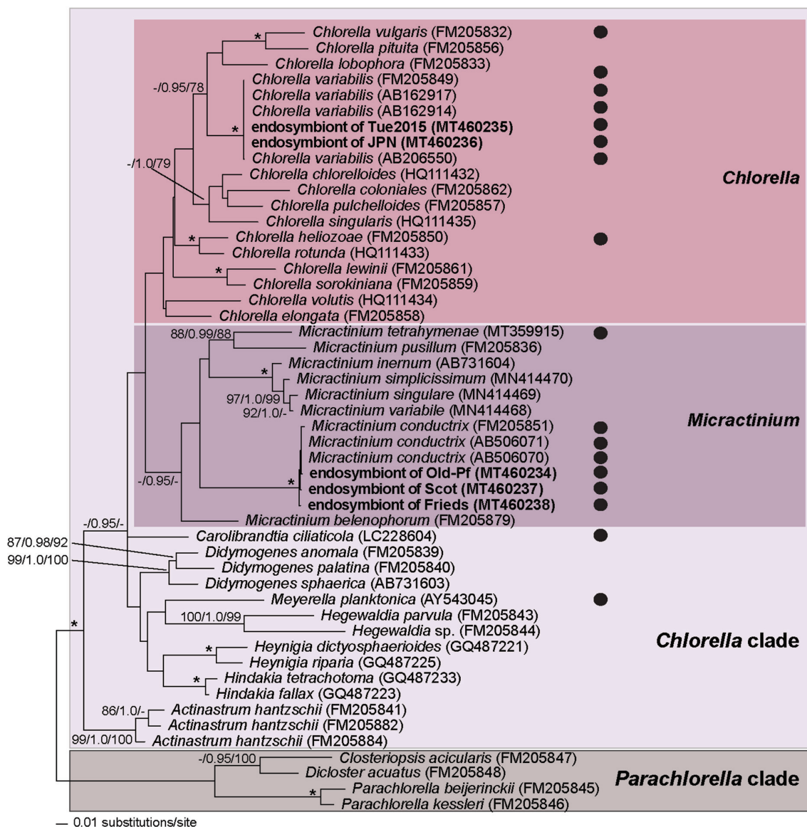
Figure 5. Molecular identification of microalgal endosymbionts. Phylogeny of members of the Chlorellaceae based on sequences covering the SSU rRNA gene and the internal transcribed spacer region spanning ITS1-5.8S-ITS2. The shown tree was inferred by the Neighbour Joining method based on 2224 aligned positions. GTR+I+G was used as evolutionary model. Bootstrap values above 70 % and Bayesian Interference values above 0.95 are indicated (ML/BI/NJ). Asterisks indicate maximum support in all analyses. Members of the Parachlorella clade were selected as outgroup. Black circles indicate species capable of living in symbiosis. The sequences marked in bold were obtained in this study.
