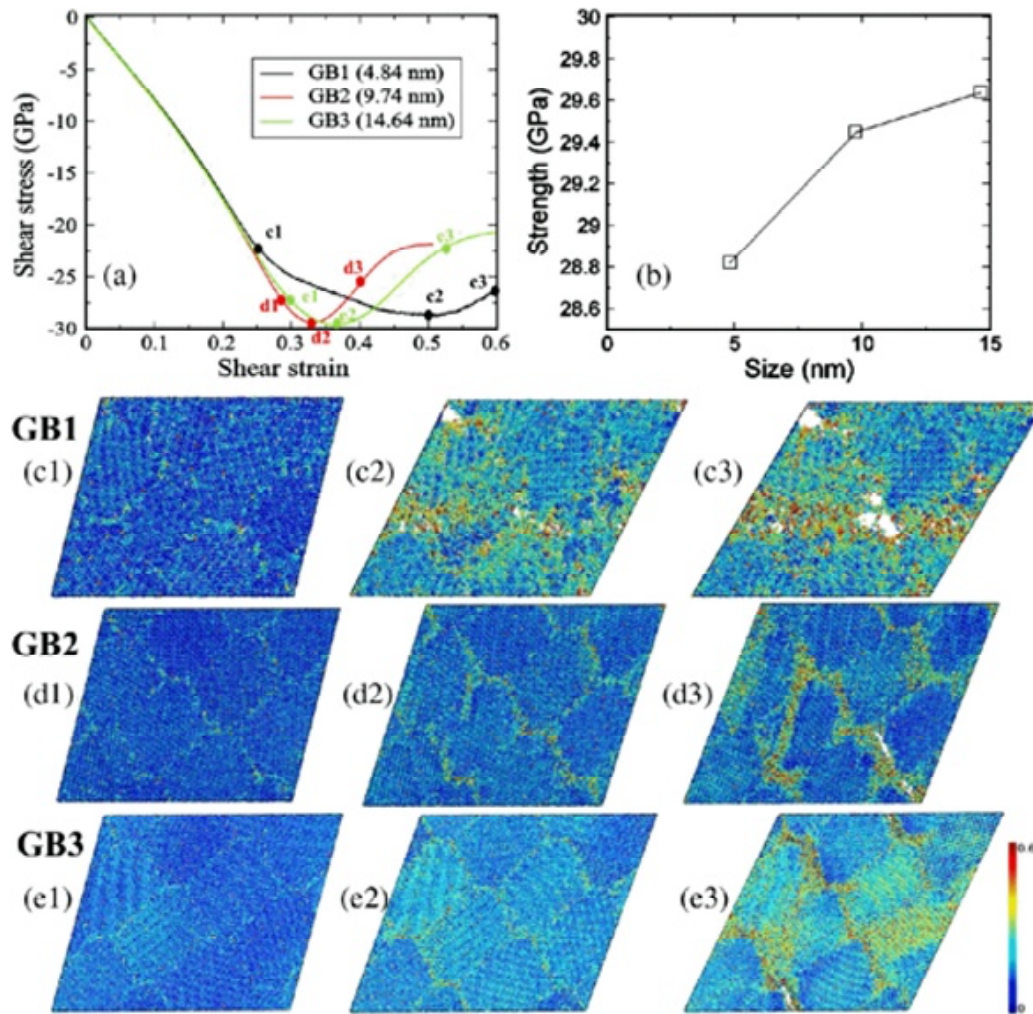
Fig. 3. (a) Stress-strain relationships of three GB models at finite shear deformation with shear rate of 0.1 \text{ ps}^{-1} . (b) The shear strength of three GB models. (c1)–(e1) Snapshots of the beginning of plastic deformation for three GB models. (c2)–(e2) Snapshots of the end of plastic deformation, reaching the maximum shear strength. (c3)–(e3) Snapshots of the cavitation formation. Atoms are colored based on their atomic shear strain. The sizes of GB3 and GB2 are 3 and 2 times larger than the size of GB1. Reproduced from Guo et al. [16], with permission. Copyright (2018), American Physical Society, https://doi.org/10.1103/PhysRevLett.121.145504 .
