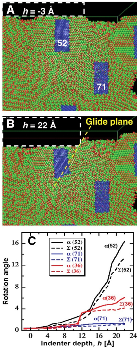
Fig. 1. Rotation of grains in nanocrystalline SiC under indentation revealed in MD simulations. (A and B) Si (green) and C (red) atoms are shown for the cases of (A) purely elastic deformation and (B) just after the onset of yielding (white dashed lines depict the position of the indenter, h is the indentation depth). Grain 52 experiences enormous shear and undergoes large rotation and deformation. (C) Rotation angle \alpha(n) and its standard deviation \Sigma(n) of selected grains with number n = 52, 71, and 36 . Grain 52 undergoes large rotation and deformation (black curve). Localization of deformation is reflected in the lack of rotation of grain 71 (blue curve). Reproduced from Szlufarska et al. [34], with permission. Copyright (2005), American Association for the Advancement of Science.
