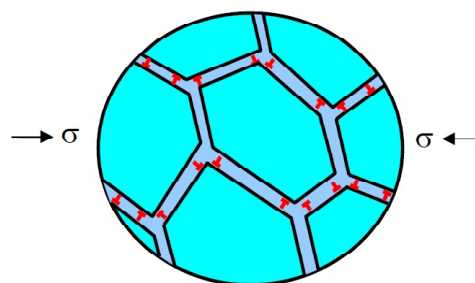
Fig. 4. A fragment of a nanocrystalline ceramic solid (under a uniform compressive stress \sigma ) where plastic deformation is realized through thermally activated grain boundary sliding. Reproduced from Sheinerman et al. [53], with permission. Copyright (2020), Elsevier.
