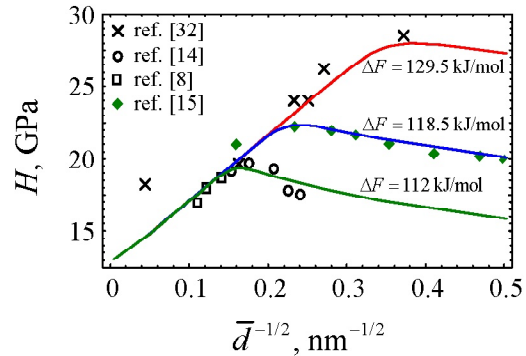
Fig. 5. Microhardness H as a function of the inverse square root of the grain size, d^{-1/2} , for various values of the activation energy \Delta F . Reproduced from Sheinerman et al. [53], with permission. Copyright (2020), Elsevier.
