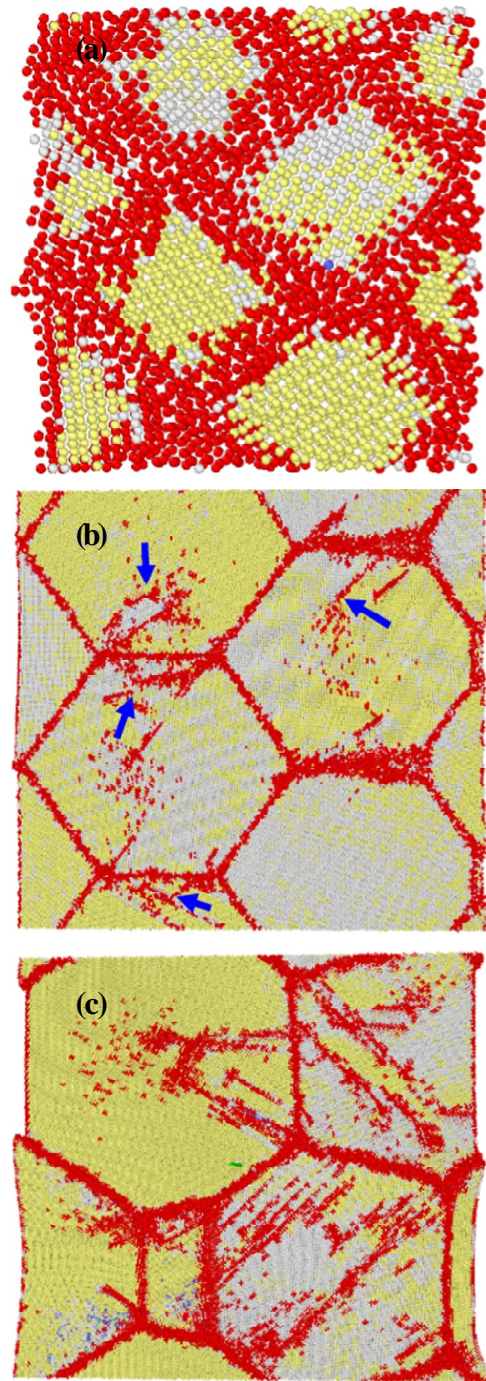
Fig. 2. The deformation microstructures at three representative grain sizes of polycrystalline WC: (a) 5.0 nm, (b) 24.0 nm and (c) 31.4 nm. The atoms (both at the grain boundaries and in the grain interiors) with higher potential are colored red, and the rest are in the HCP structure. The arrows in (b) show the sites of dislocation intersections. Reproduced from Feng et al. [35]. Copyright (2017), Institute of Physics Publishing.
