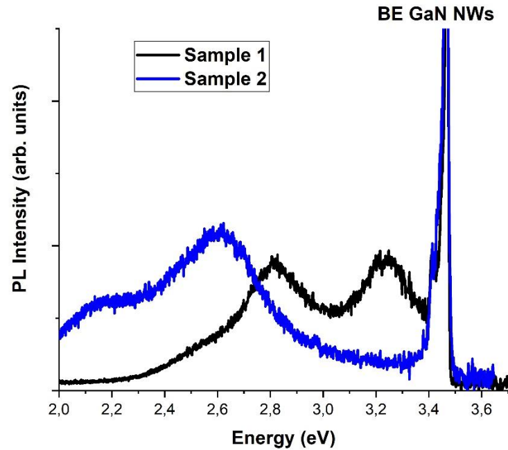
Fig. 2. PL spectra of GaN nanowires with fifteen InGaN quantum disks.
