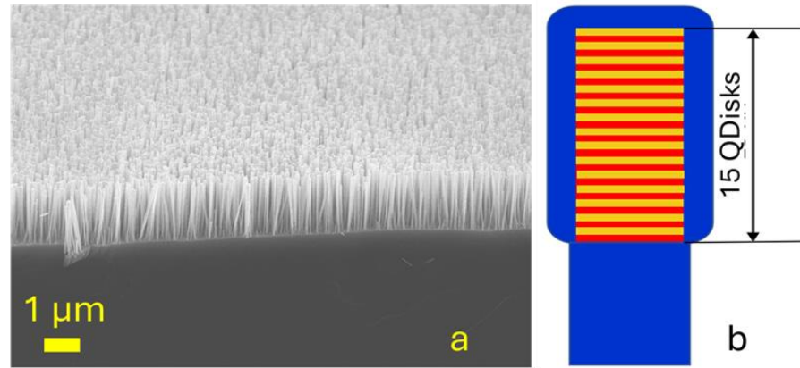
Fig.1. a) SEM image of GaN NWs with InGaN superlattice b) a scheme of the NW with the superlattice structure.
