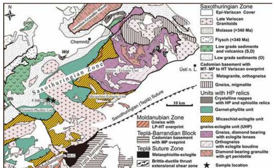
The schematic geological map of the Saxothuringian Zone according to Faryad & Kachlík (2013).
