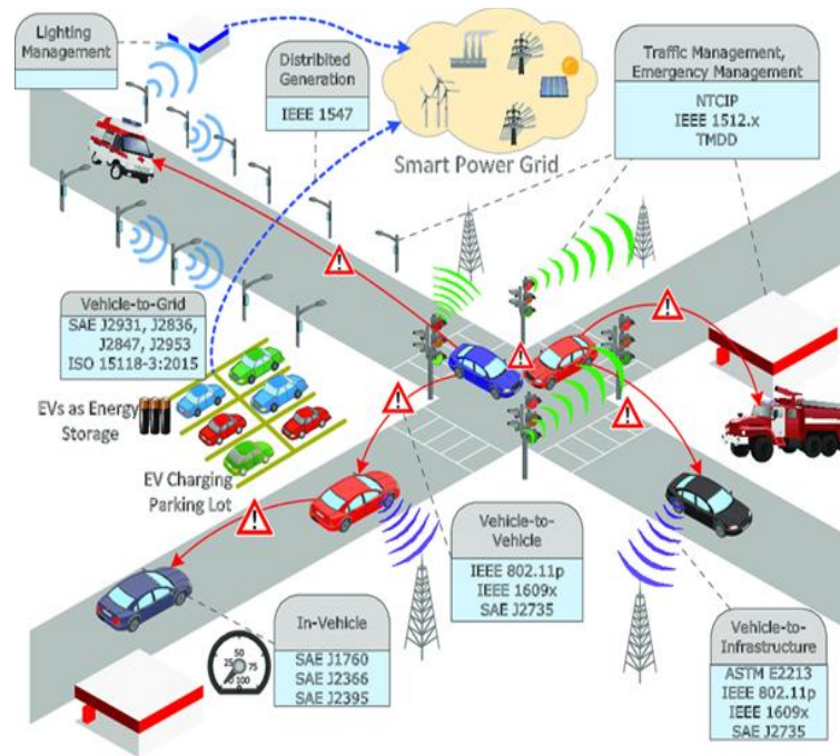
Fig. 2. ITS architecture.
