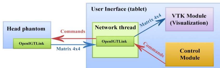
Fig. 3. Redesigned network architecture
