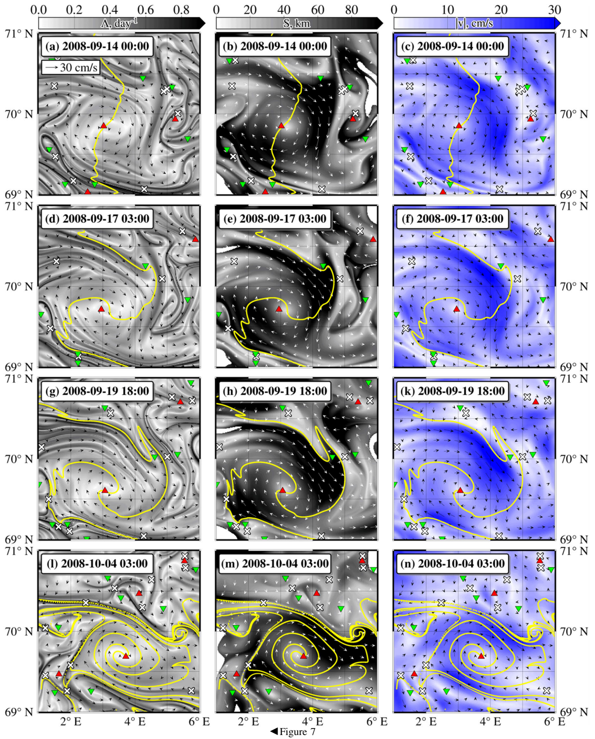
Individual slides “Experiment with a Segment”: the evolution of the Segment against the background of the Lofoten Vortex: \Lambda -maps (left column), S -maps (central column), and the velocity field (right column) for a layer of 50 m according to ROMS data. The red triangles indicate the centers of anticyclones, and the green ones indicate cyclones. The crosses indicate hyperbolic points
