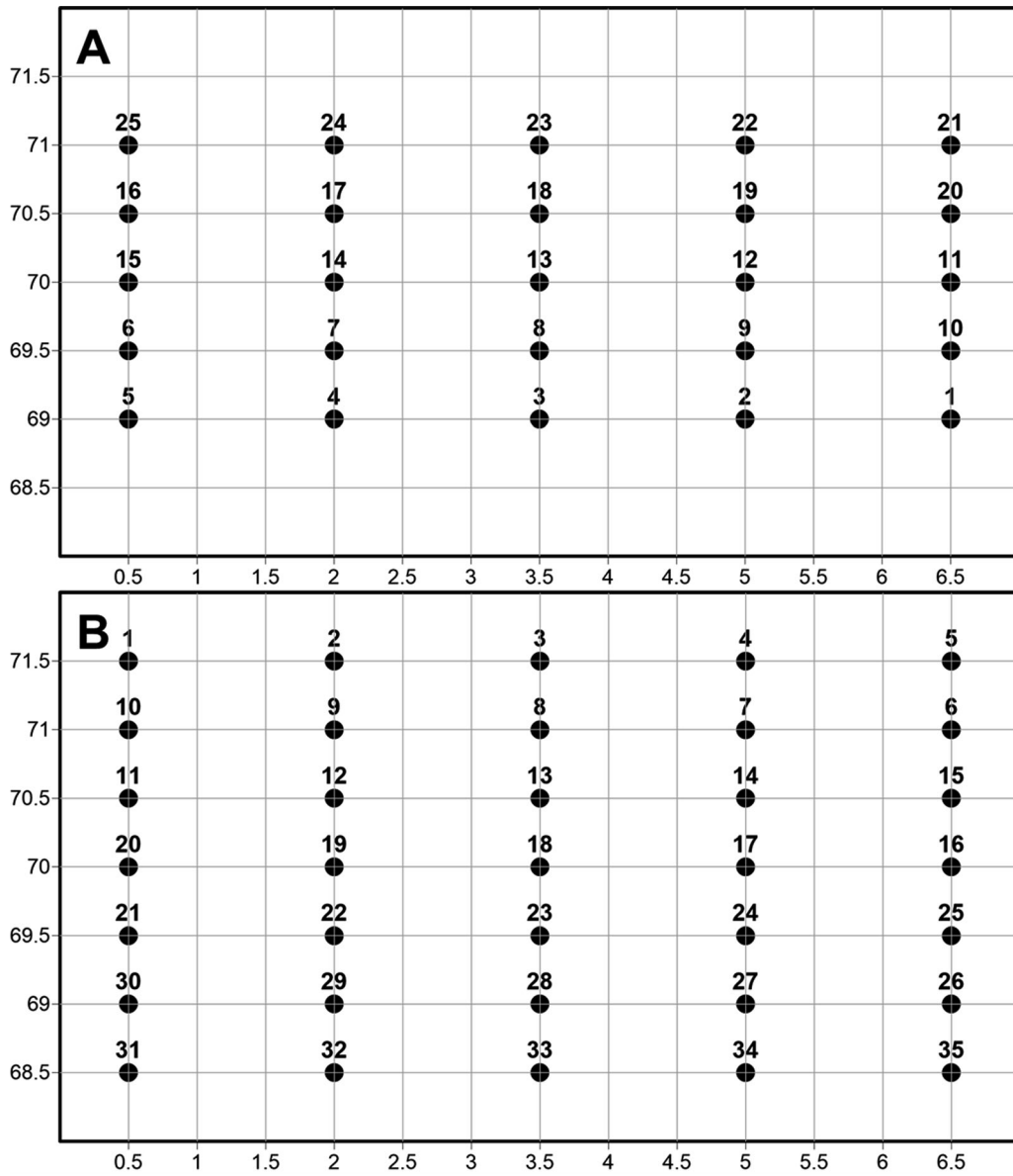
Figure 11 Diagram of CTD stations in the September 1987 expedition (A) and the September 1989 and 1990 expeditions (B)
