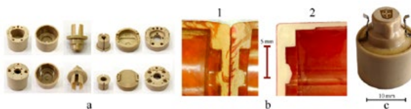
Figure 1. a – The appearance of small-sized parts; b – comparison of imperfection degree of the part made of pressing moulding material AG-4V (1) and injection moulding material TERMORAN PPS GF-40 (2) using the color capillary defectoscopy method; c – the appearance of the power source for electronic-mechanical devices.
