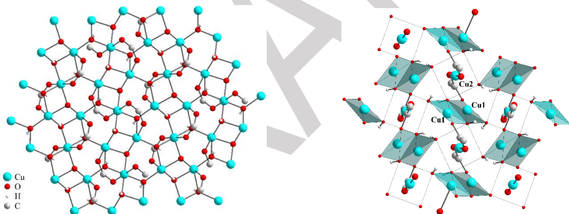
Figure 1. A fragment of the structure of \text{Cu}_3(\text{CCl}_3\text{COO})_2(\text{OH})_4 (left) and [\text{Cu1Cu1}] «dimers» having a supposed magnetic exchange (right). Trichloromethyl groups are hidden.
