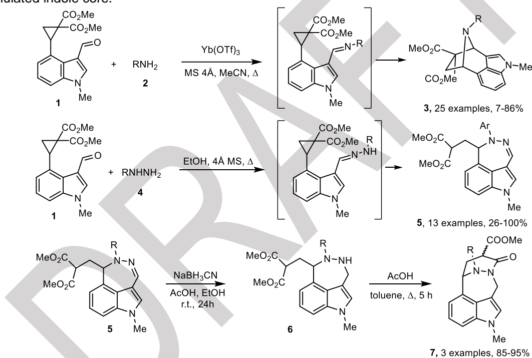
Scheme 1. Pathways of new types of peri -annulated indoles synthesis.
