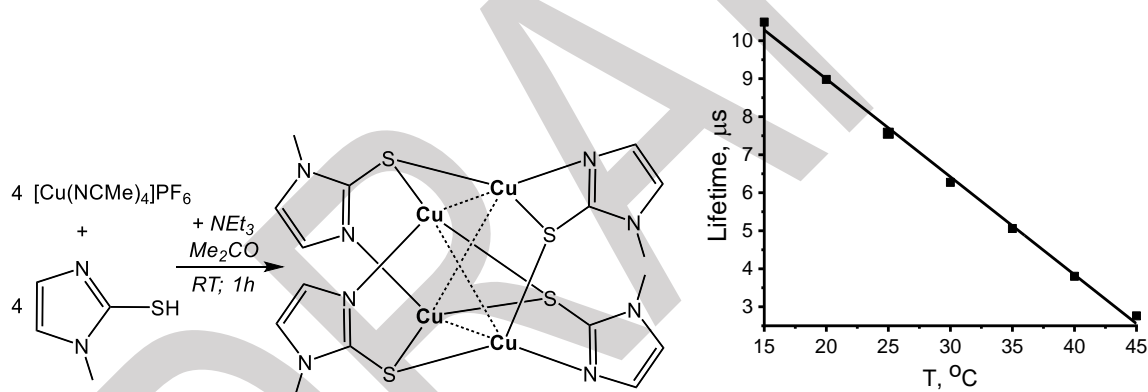
Figure 1. Scheme of the synthesis of the copper(I) cluster (left) and temperature dependency of the excitation state lifetime of this complex (right)
