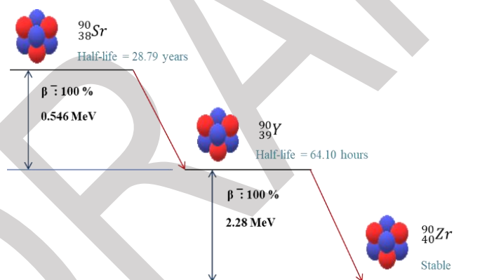
Scheme 1. ^{90}\text{Sr} in equilibrium with its ^{90}\text{Y} daughter ( E_{\max} = 2280 \text{ keV} and t_{1/2} = 64.10 \text{ hours} ).
