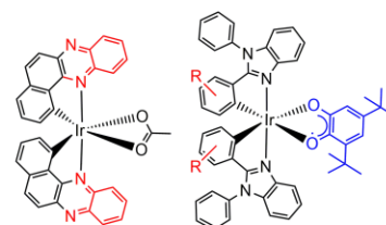
Scheme 1. Main strategies for tuning absorption in cyclometalated iridium(III) complexes probed in this work
