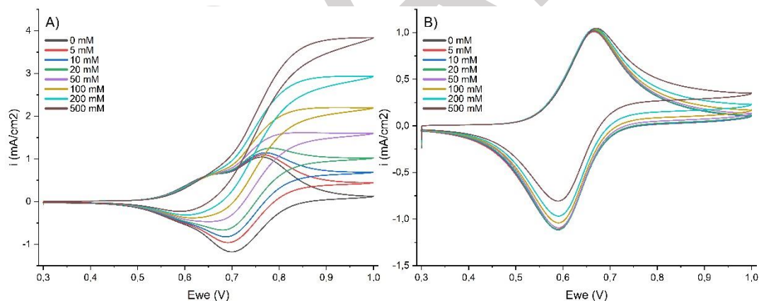
Scheme 2. CVA of poly-TEMPO-pyrrole at different glucose concentrations in the electrolyte composition: 200 mM phosphate buffer, pH = 7.4 (A), 100mM NaClO 4 , 100 mM phosphate buffer, pH = 7.4 (B). Sweep speed 50 mV/s
