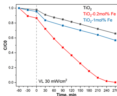
Figure 1. Photocatalytic performance of the 0.2 mol% Fe 3+ -doped sample for the degradation of Orange II under visible light irradiation.
