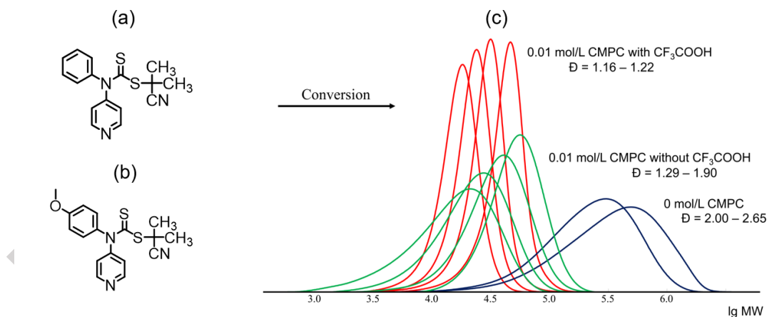
Scheme 1. (a) Structure formula of CMPC; (b) structure formula of CMPCM; (c) SEC curves normalized by the unit area for polymerization of styrene in presence of CMPC
