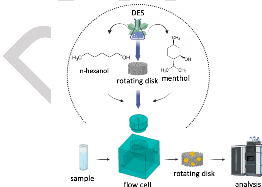
Scheme 1. Flow extraction device
