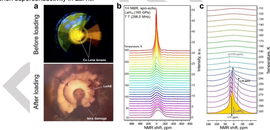
Scheme 1. 1 H NMR in La polyhydrides. (a) Photographs of the anvil culet with sputtered Lenz lenses before and after loading and compression to 165 GPa. (b) Stack of 1 H NMR spectra recorded in a cooling cycle from 300 K to 10 K in steps of 10 K. The curves correspond to the signal magnitude. (c) Zoom in of the 1 H NMR signal as a function of temperature.
