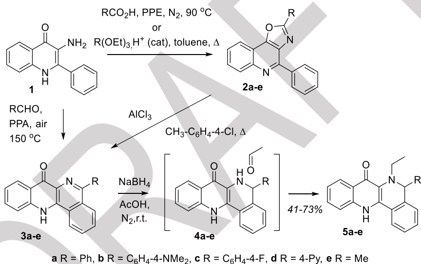
Scheme 1. Synthesis of 6-ethyl-6,12-dihydrodibenzo[ b,h ]-1,5-naphthyridin-7(5 H )-ones 5a-e .
