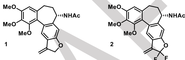
Scheme 1. Active dihydrofuranoalcolcolchicinoids.
