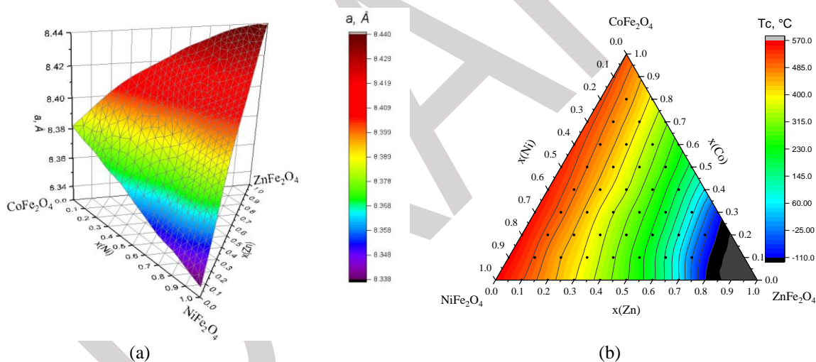
Scheme 1. Unit cell parameters (a), Curie temperature (b) of \text{Ni}_x\text{Zn}_y\text{Co}_{1-x-y}\text{O}_4 ( x=0-1 ) system
