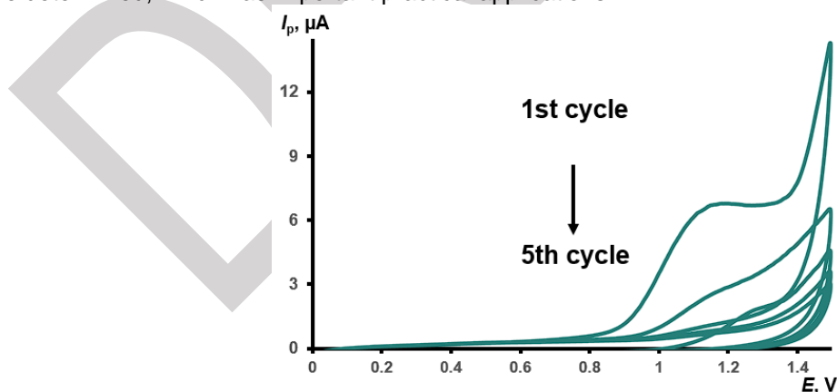
Figure 1. Cyclic voltammograms of electropolymerization of PEDOT film.
