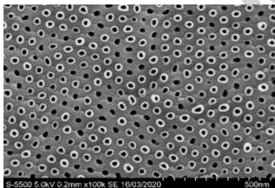
Figure 1. SEM image of porous anodic alumina membrane with carbon nanotubes (a);
