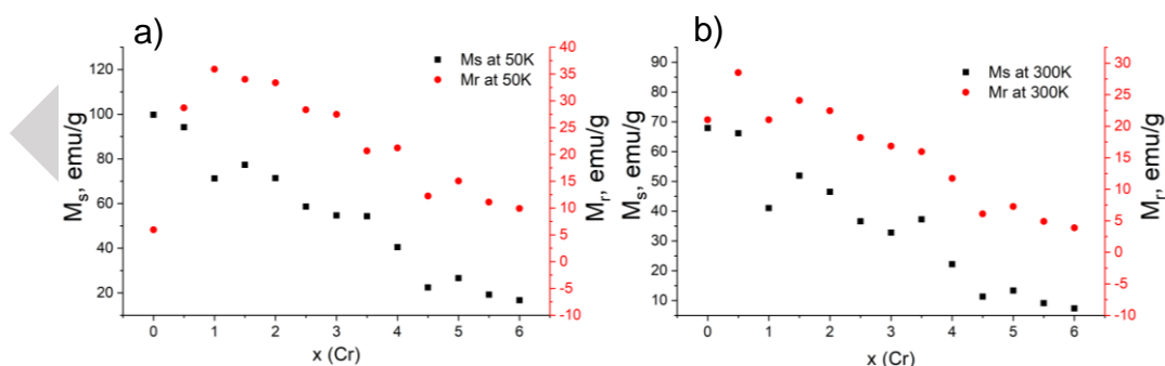
Figure 1. Dependencies on Cr concentration of a) M_s and M_r ; at 50K b) M_s and M_r at 300K
