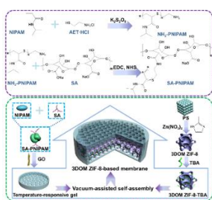
Scheme 1. Preparation of the 3DOM ZIF-8-based membrane
