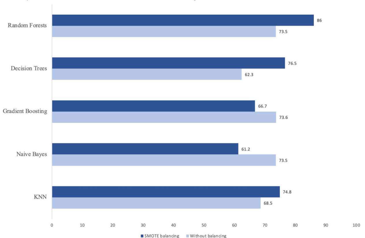
Figure 1. Comparison of Machine Learning Model Accuracy with and without SMOTE Balancing
