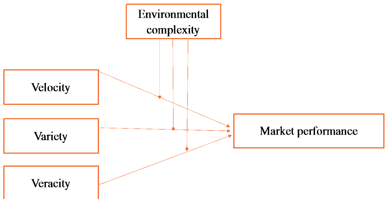
Figure 1. Theoretical model
