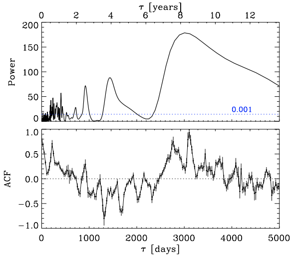
Fig. 8. Power spectrum of the discrete Fourier transform ( top ) and auto-correlation function ( bottom ) obtained from the historical R -band light curve. In the top panel the blue dotted line indicates the level above which the significance is better than 0.001.
