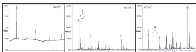
Fig. 1. Chromatograms of the products obtained at different temperatures
