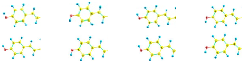
Fig. 1. Resveratrol Conformers
