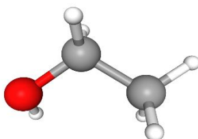
Fig. Model of the ethanol molecule
