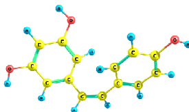
Fig. 2. Structure of cis-resveratrol
