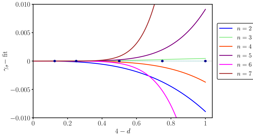
Figure 5: Comparison of \gamma_\sigma bootstrap data with unresummed epsilon expansion (3.5) in the region 4 > d > 3 for truncations of the series to order n = 2, \dots, 7 (see color legend). All quantities have been subtracted by the best fit values (see (3.6)).
