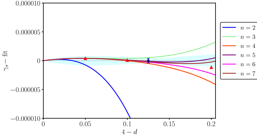
Figure 6: Comparison of \gamma_\sigma data minus best fit in the region 4 > d > 3.8 , between bootstrap (blue circle) and unresummed epsilon expansion (3.5) with different truncations of the perturbative series (cf. Fig. 5). The red triangles are the results of the bootstrap navigator method [21]. The cyan shaded area is the fit error.
