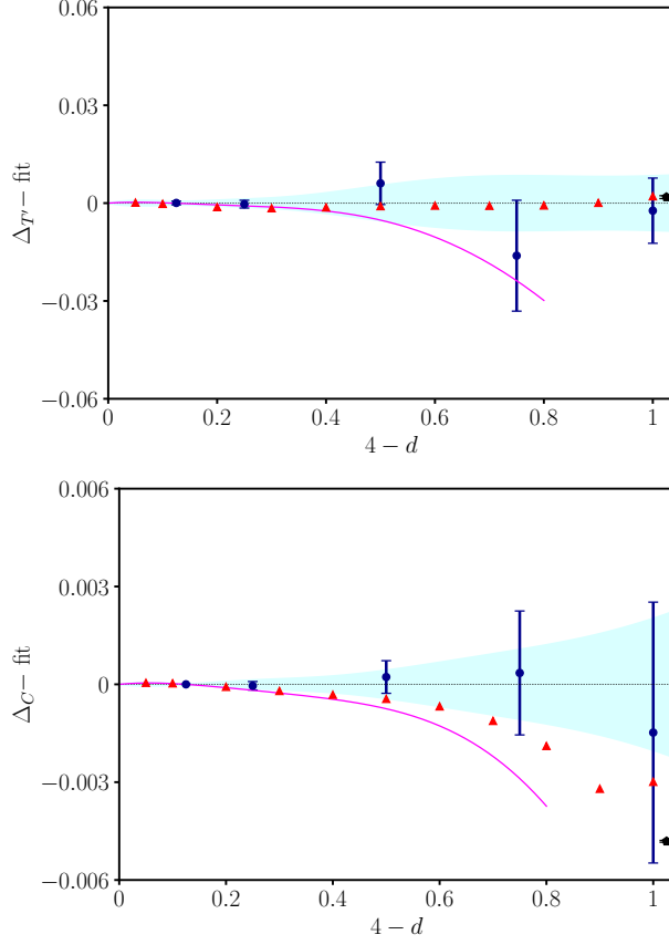
Figure 18: Comparison of scaling dimensions minus best fit for T' , C fields: bootstrap (blue round points), navigator method [21] (triangle red points), 3-correlator bootstrap at d = 3 [48] (black pentagon) and unresummed epsilon expansion [27, 32, 58, 59] (magenta solid line).
