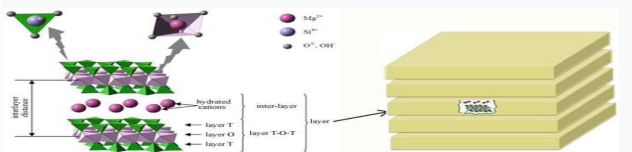
Figure 3. vermiculite structure
