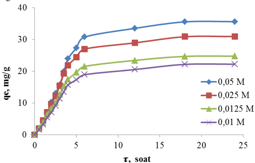
Fig. 2. Graph of the time dependence of the absorption of \text{Cu}^{2+} ions into an ion exchange obtained on the basis of vermiculite.
