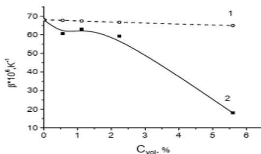
Fig. 2. Comparison of calculated (1) according to equation (3.7) and experimental (2) and dependences of the CTE of the composite on the concentration of copper powder.
