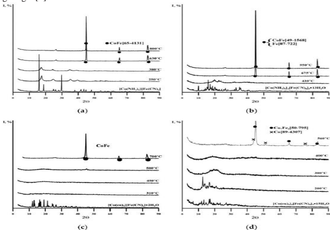
1-rasm. DCC ning XRD naqshlari va ularning argondagi termoliz mahsulotlari: a) [\text{Co}(\text{NH}_3)_6][\text{Fe}(\text{CN})_6] ; b) [\text{Co}(\text{NH}_3)_4][\text{Fe}(\text{CN})_6]_3 \cdot 13\text{H}_2\text{O} ; c) [\text{Co}(\text{en})_3][\text{Fe}(\text{CN})_6] \cdot 2\text{H}_2\text{O} ; d) [\text{Co}(\text{en})_3]_4[\text{Fe}(\text{CN})_6]_3 \cdot 15\text{H}_2\text{O} .
