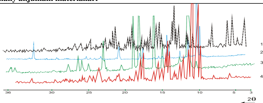
1-rasm. Rentgenogramma: 1-CS(NH 2 ) 2 ; 2-CO(NH 2 ) 2 ; 3-Ca(CH 3 COO) 2 ·H 2 O u 4-CaAKTK·0,5H 2 O
