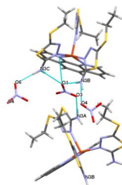
Fig. 3. Intramolecular and intermolecular hydrogen bonds.
