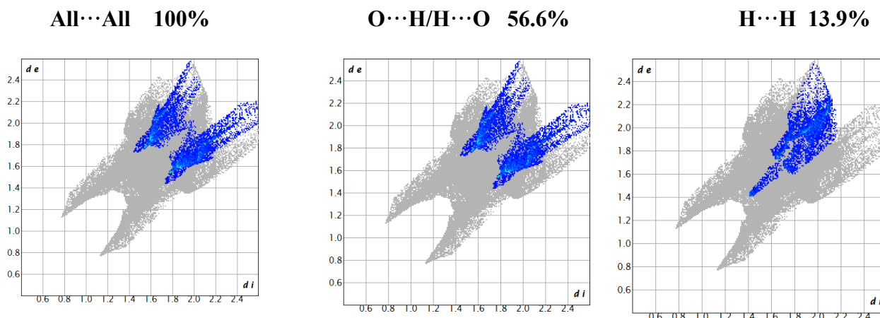
Figure 4. The full 2D fingerprint plots for PNA copper complex showing all interactions and delineated into O...H/H...O, H...H, C...O/O...C, C...H/H...C and O...O interactions. The d_i and d_e values are the closest internal and external distances (Å) from given points on the Hirshfeld surface contacts.
