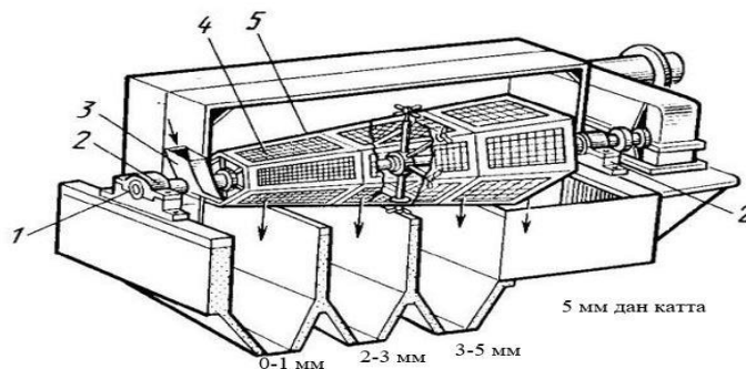
1-rasm. Sito-burat SM-237A: 1- gorizontaal val, 2 - podshipniklar, 3 –xom ashyo kirish qismi, 4 –turli o’lchamdagi setkalar, 5 –setkalarining ramalari.
