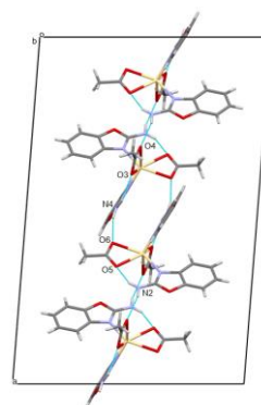
Fig. 2. Formation of the columns in the crystal structure of the complex.
