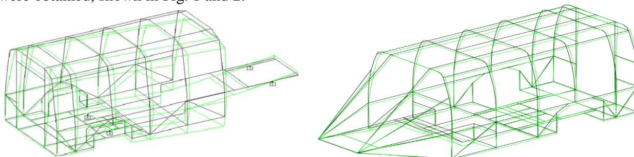
Fig.1. A picture of the deformed state of the frame elements with a skin made of steel plates with double-sided galvanizing under load F=10000 H
