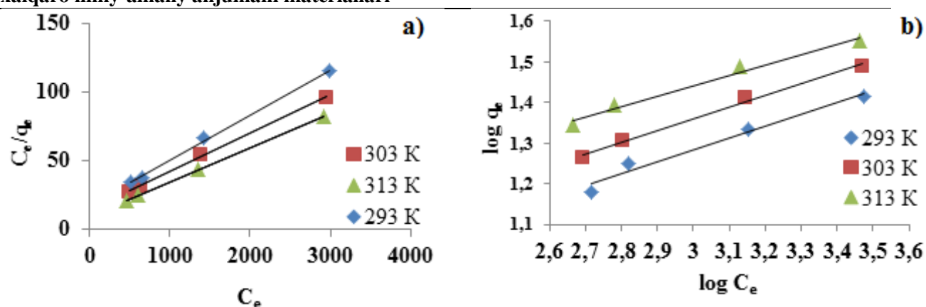
Fig. 4 Graphs of Langmuir (a) and Freundlich (b) isotherm models of sorption of \text{Cu}^{2+} ions on vermiculite-based ion exchange
