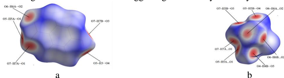
Fig.2. View the three-dimensional Hirshfeld surface for PHBA anion (a) and [Ni(H_2O)_6] cation (b) of the title compound 1 plotted over d_{norm} in the range of -0.4180 to 1.3344 a.u.
