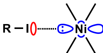
Figure 1. The C-I\cdots Ni^{II} XBs.
