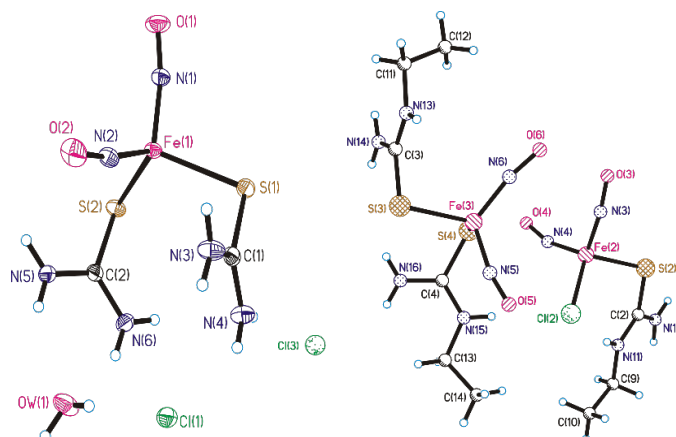
Figure 1. Molecular structure of the complex 1 and 2.
