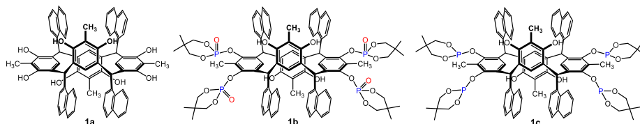
Figure 1. Initial compounds.
