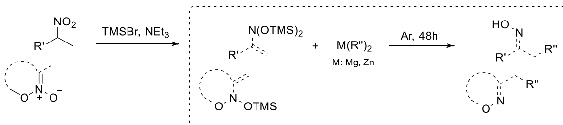
Figure 1. Reaction
