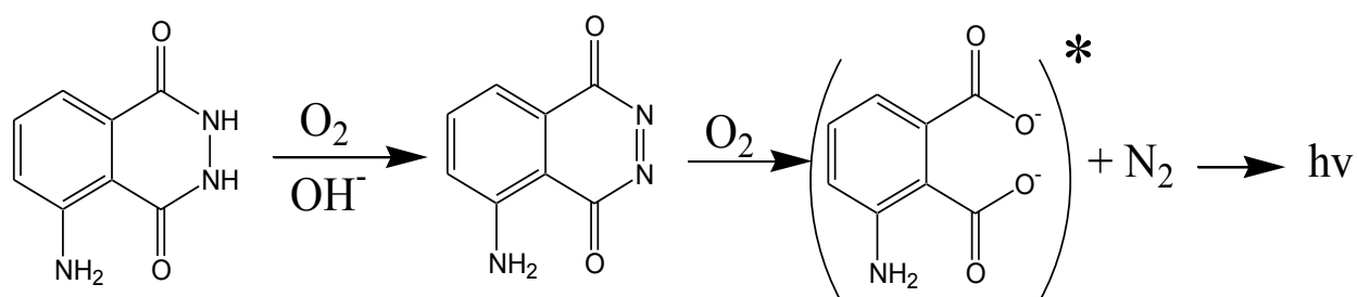
Figure 1. Luminol oxidation reaction.
