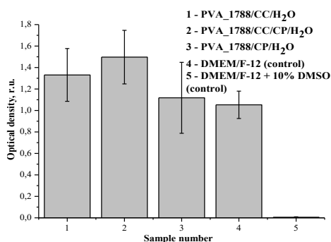
Figure 1. Stromal cells metabolic activity according to MTT-test.
