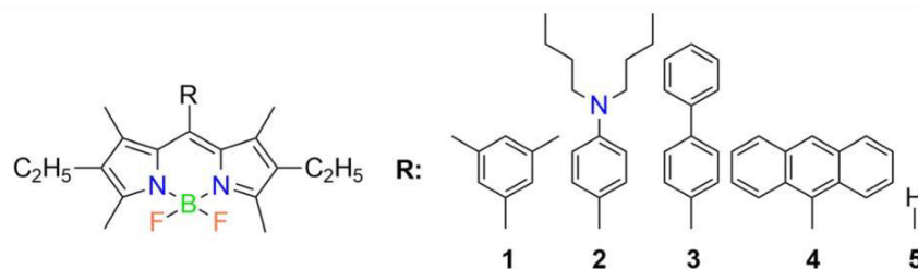
Figure 1. Investigated BODIPYs.
