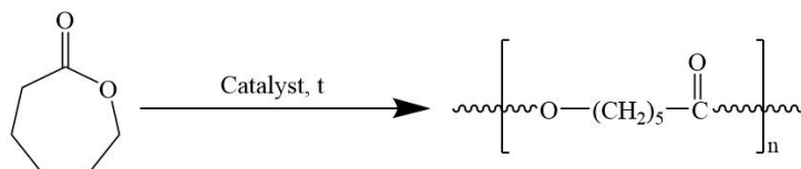
Figure 1. Scheme of polymerization of \epsilon -caprolactone
