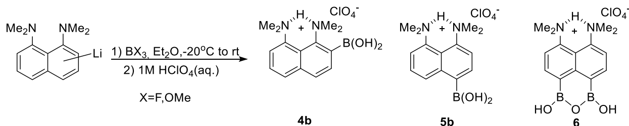
Scheme 2. Synthesis of ortho - and para - 1,8-bis(dimethylamino)naphthalenylboronic acids.
