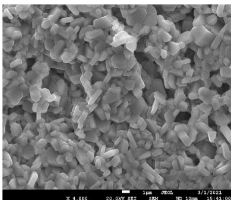
Figure 1. SEM images of BaFe 11,9 Mn 0,1 O 19 of the sample.
