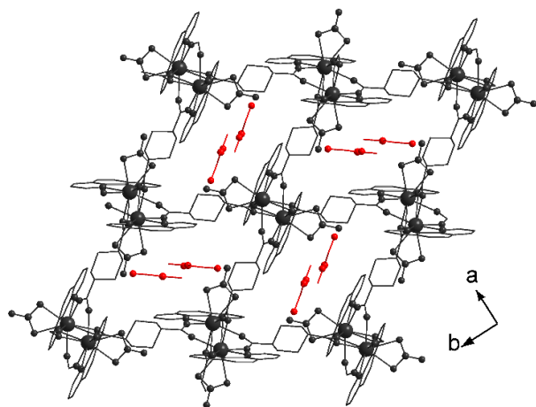
Figure 3. The coordination network [\text{Ln}(\text{phen})(\text{NO}_3)(\text{chdc})] (black) and the location of guest DMF molecules (red).
