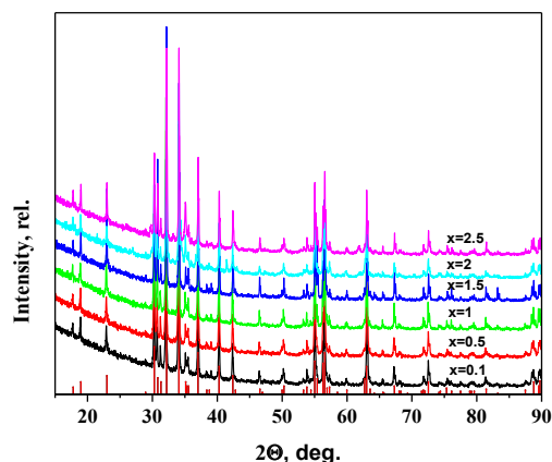
Figure 2. Powder X-ray diffraction patterns for synthesized samples.
