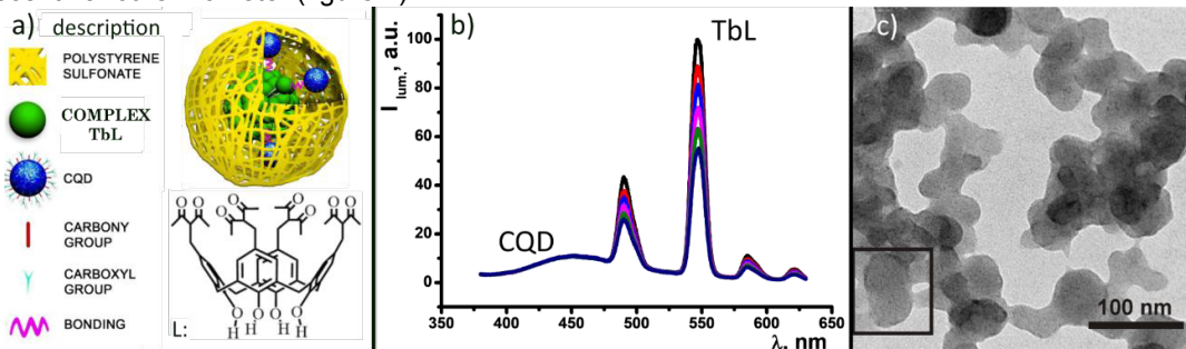
Figure 1. Schematic description of hybrid nanoparticle and structure of ligand of complex [TbL] (a), emission spectra of this nanoparticles ( I_{\text{ex}} = 360 \text{ nm} ) as a function of temperature (b), TEM image of dried colloids (c)
