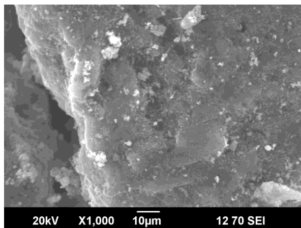
Figure 1. SEM micrograph of the MnO 2 /CNT composite.
