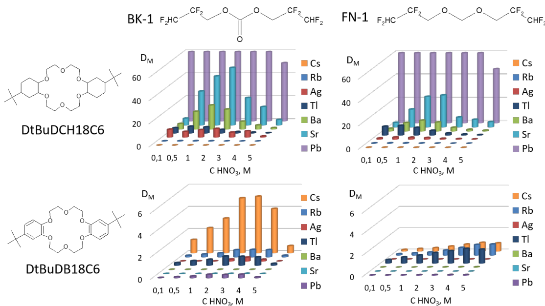
Figure 1. Dependence of the distribution coefficients of metals (Pb(II), Sr(II), Ba(II), Tl(I), Ag(I), Rb(I), Cs(I)) on the concentration of HNO 3 for the extraction system DtBuDCH18C6 & DtBuDB18C6 0.05 M in BK-1 & FN-1.
