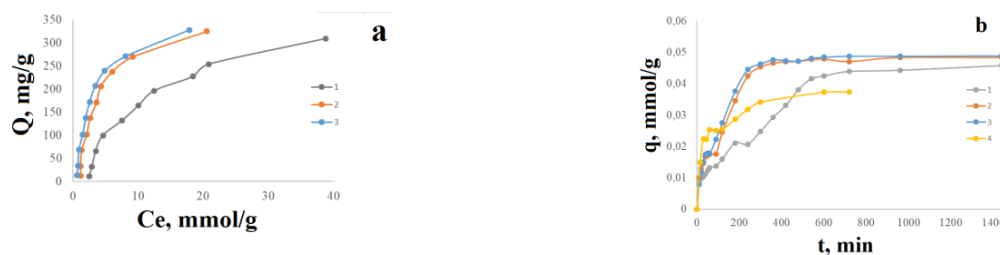
Figure 1. a-Isotherms of sorption of Congo red on LDHs; b- Kinetic curves of sorption of Congo red on LDH: 1- MgCo/AlFe-air (T=25°C), 2-MgCo/AlFe-air (T=35°C), 3-MgCo/AlFe-air (T=45°C), 4-MgCo/AlFe-Ar (T=25°C)
