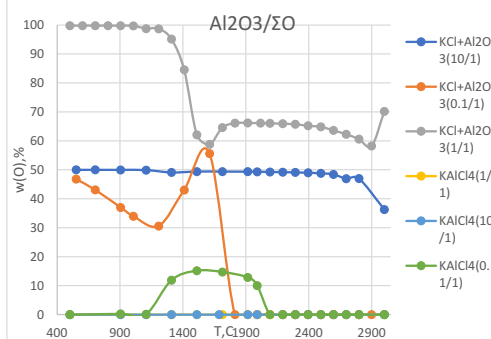
Figure 3. aluminum oxide produced in the systems
