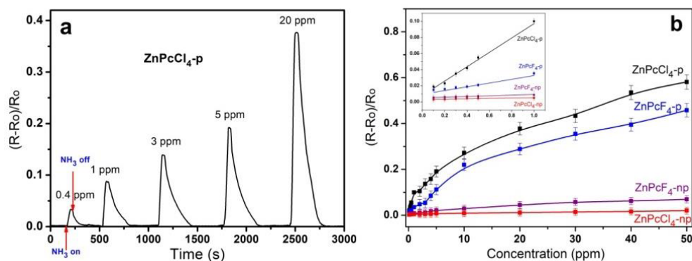
Figure 1. (a) Real-time sensor response of a ZnPcCl_4 -p film to ammonia, measured at RH 10 % and 25 °C. (b) Dependence of the sensor response of ZnPcF_4 -np, ZnPcF_4 -p, ZnPcCl_4 -np, and ZnPcCl_4 -p sensing layers on ammonia concentration.
