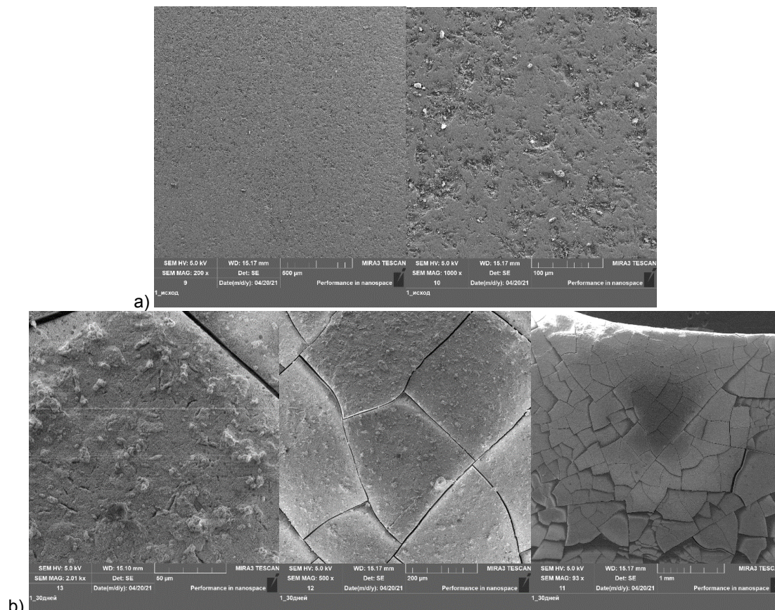
Figure 1. SEM micrographs of Compound #1 (a) before and (b) after immersed in SBF for 30 days.
