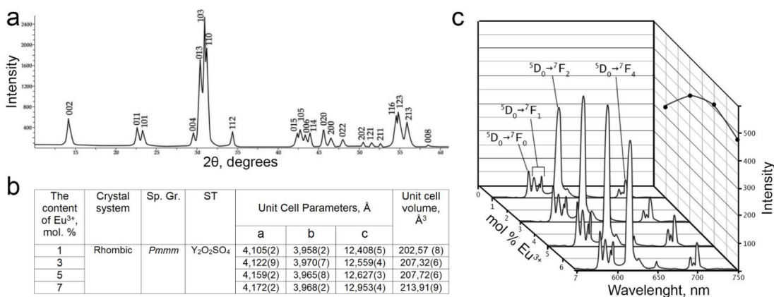
Figure 1. XRD pattern (a), crystal parameters (b) and emission spectra (c) of Lu 2 O 2 SO 4 :Eu 3+ samples
