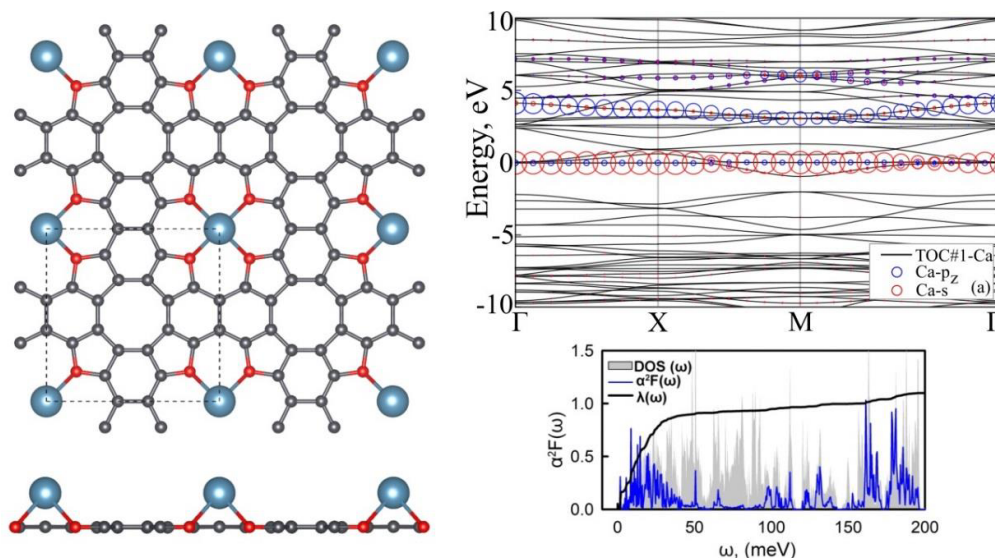
Figure 1. Structure and properties of organometallic polymers based on tetraoxa[8]circulene and calcium atoms. DOS, \alpha^2F(\omega) , \lambda(\omega) and \omega are phonon density of states, Eliashberg spectral function, electron-phonon coupling and frequency, respectively.
