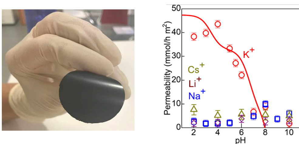
Figure 1. A photograph of free-standing GO-PA membrane. Ionic permeation of GO-PA membranes as a function of pH measured separately for K^+ and Na^+ .
