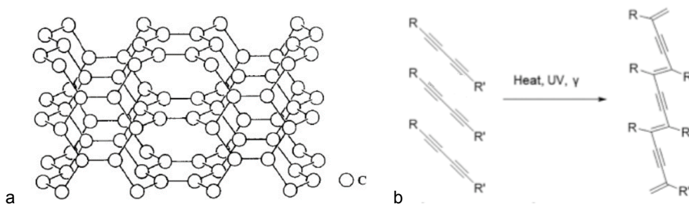
Figure 1. Structures of tetragonal forms of carbon (a), topochemical polymerization of diacetylenes in the solid state (b)
