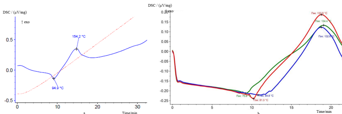
Figure 1. Thermal analysis of adhesive prepregs.
