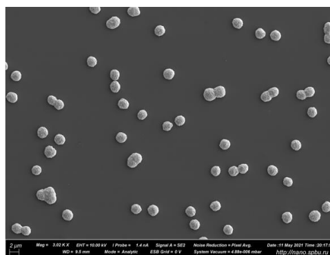
Figure 2. Silver microparticles arrays.
