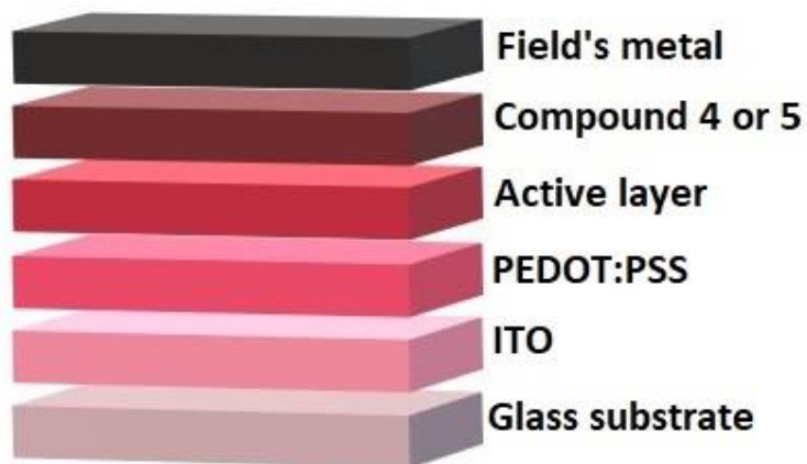
Figure 1. Scheme of photovoltaic cells.
