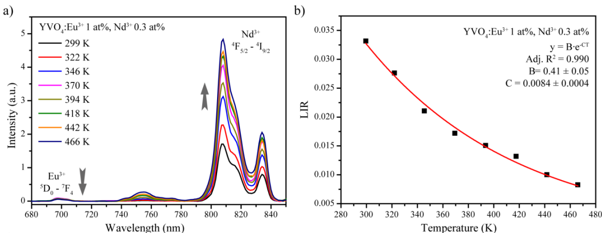
Figure 1. Emission spectra of a) co-doped YVO 4 :Eu 3+ 1 at.%, Nd 3+ 0.3 at.% nanoparticles measured at various temperatures; b) LIR evolution of co-doped YVO 4 :Eu 3+ 1 at.%, Nd 3+ 0.3 at.% nanoparticles.
