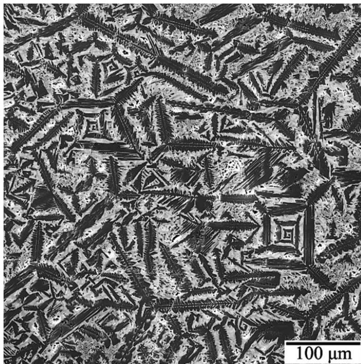
Figure 1. – SEM-image of crystallized sample at system \text{LaB}_6\text{-NbB}_2\text{-W}_2\text{B}_5
