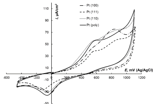
Figure 1. CVs of Pt electrodes in blood plasma.
