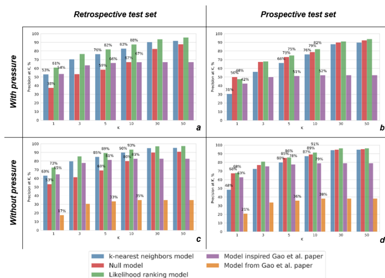
Figure 1. Cumulative histograms of the percentage of test sets reactions for which at least one of experimental reaction conditions were found within the top of a sorted list of predicted conditions of size K. Note that prediction of pressure is ignored on the histograms c and d
