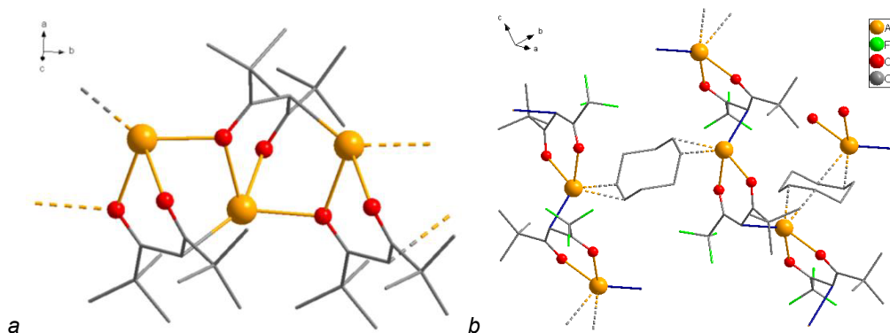
Figure 1. Ag(I) coordination polymers: (a) [Ag(tBuCOCHCOtBu)]_{\infty} (b) [Ag_2(cod)(tBuCOCHCOCF_3)_2]_{\infty} . Hydrogen atoms are omitted for clarity.
