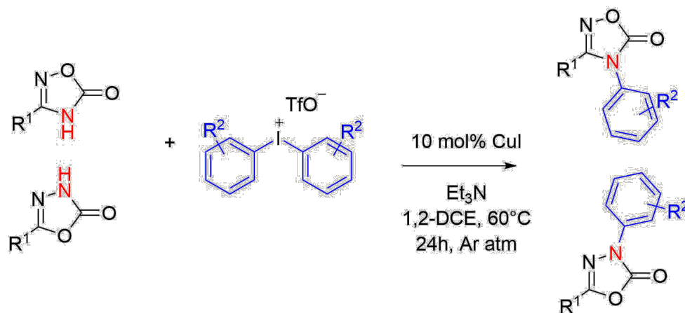
Figure 1. Reaction.
