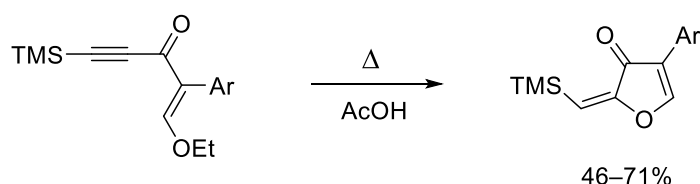
Figure 1. Cyclization of alkenynones into furanones
