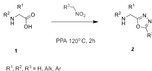
Figure 1. Reaction.
