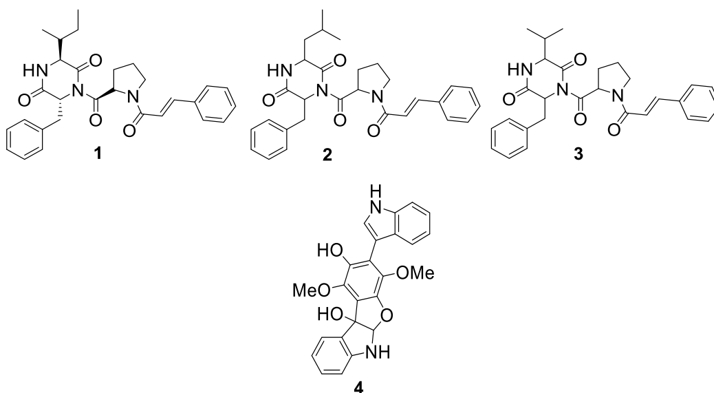
Figure 1. Structures of compounds 1-4
