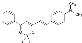
Figure 1. 2,2-difluoro-4-(p-dimethylaminostyryl)-6-phenyl-1,3,2-dioxaborine
