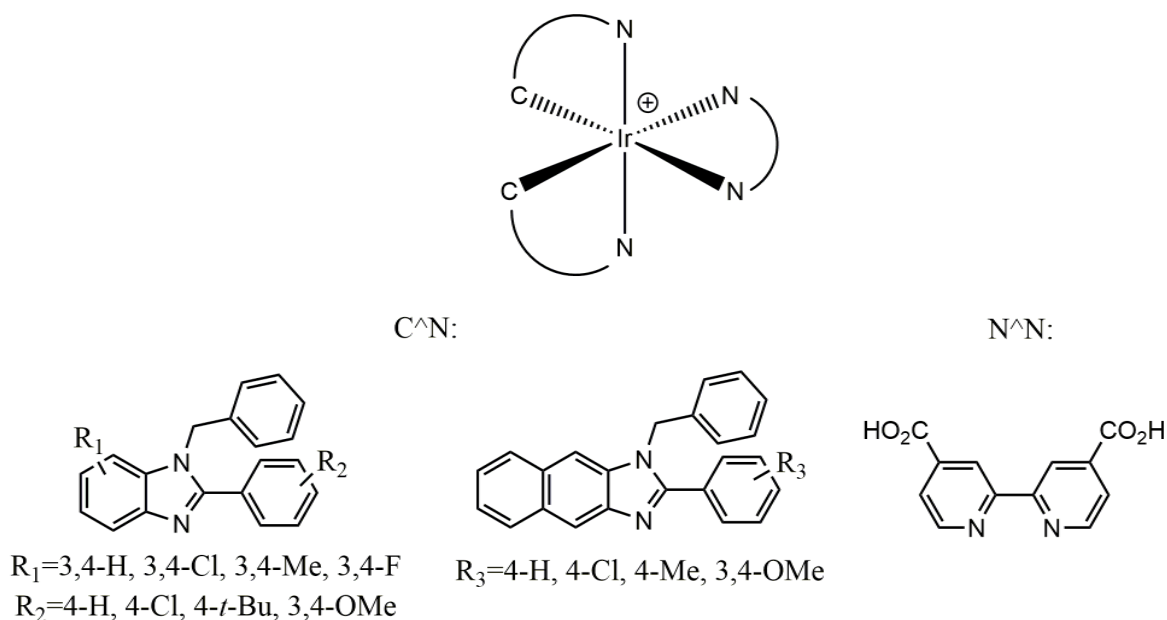
Figure 1. Complexes studied in this work
