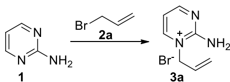
Figure 1. Synthesis of 1-allyl-2-aminopyrimidinium bromide ( 3a )
