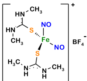
Figure 1. [\text{Fe}(\text{SC}(\text{NHCH}_3)_2)_2(\text{NO})_2]\text{BF}_4 structure.
