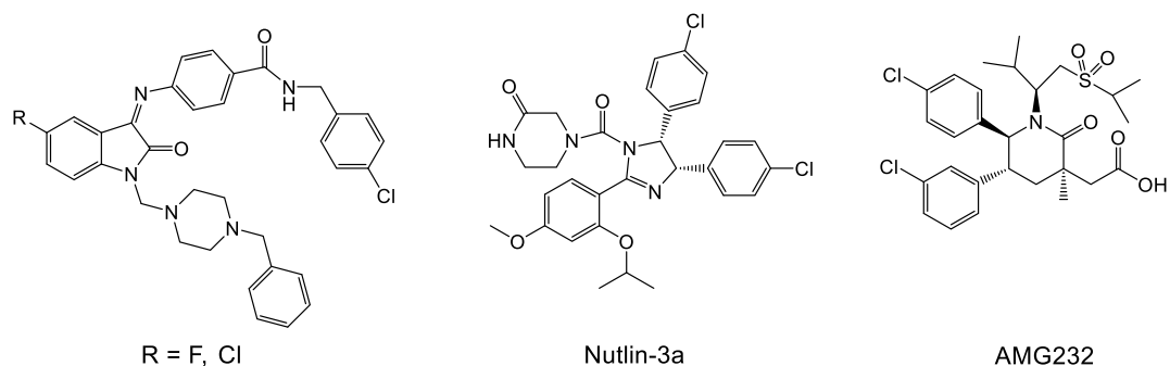
Figure 1. Structures of p53-MDM2 protein-protein interaction inhibitors
