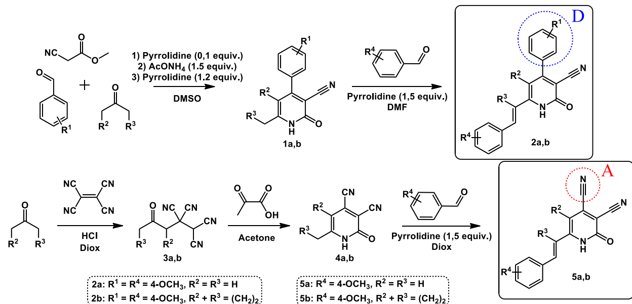
Figure 1. Synthesis of styrylpyridones
