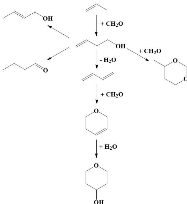
Figure 1. Reaction scheme.
