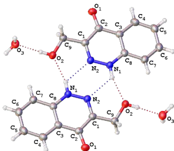
Figure 2. Dimer in crystal 16
