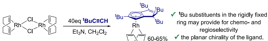
Figure 1. Formation of ( t Bu 4 Cp)Rh(cyclooctadiene).
