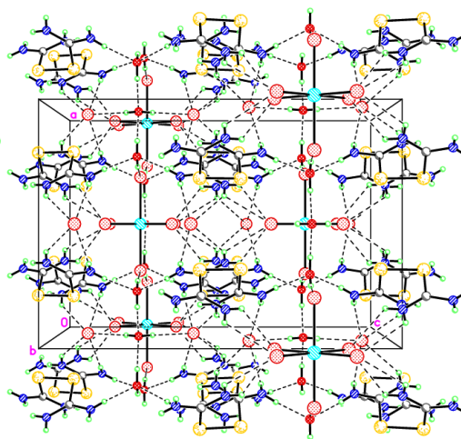
Fig. 2. The system of hydrogen bonds
