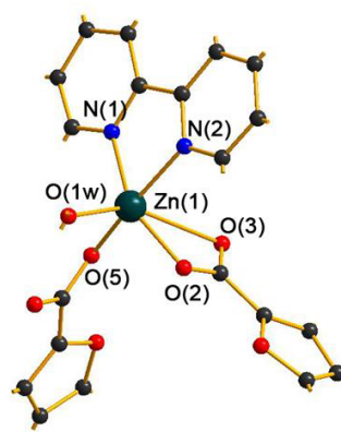
Figure 2. [Zn(fur) 2 (2,2'-bpy)]
