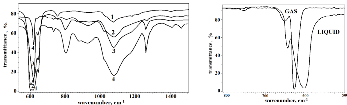
Figure 1. Spectra fragments of SiCl 4 in Si-Cl stretching region
