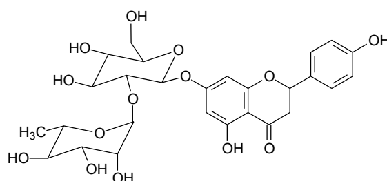
Figure 1. Naringin structure
