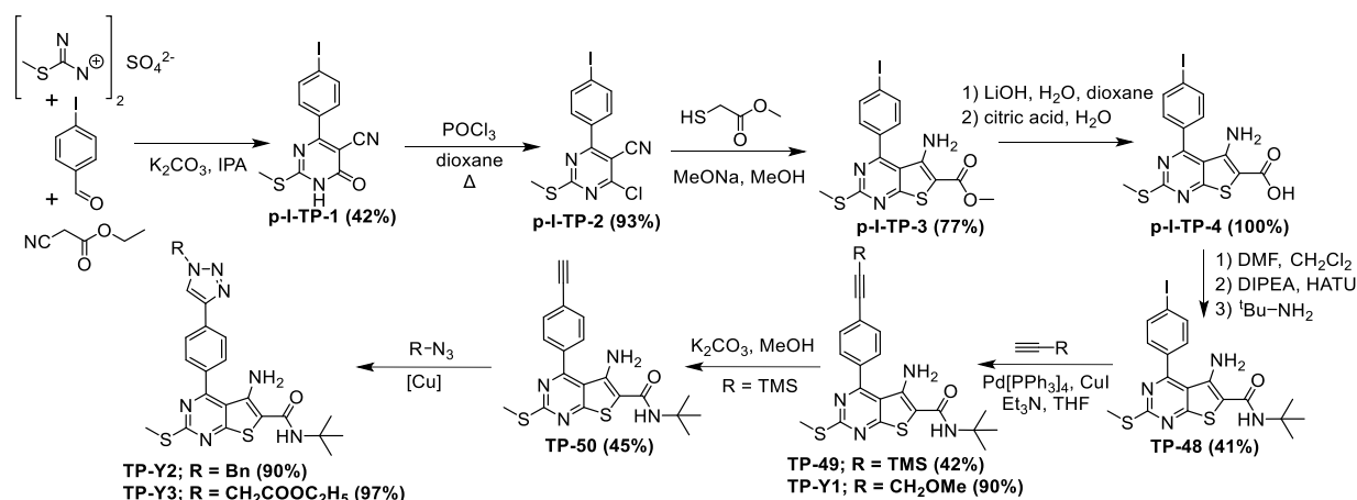
Figure 1. Synthesis Scheme.
