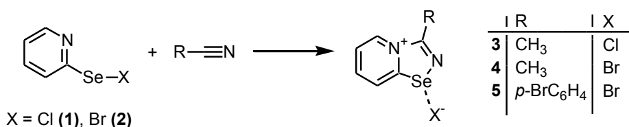
Figure 1. Synthesis of 3-5 .
