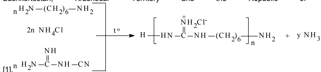
Figure 1. Reaction.
