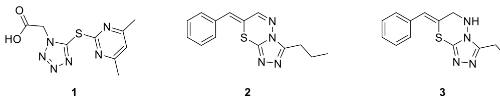
Figure 1. Synthesized compounds
