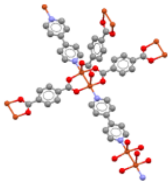
Figure 1. Structure of 1 .
