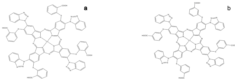
Figure 1. Research objects:
