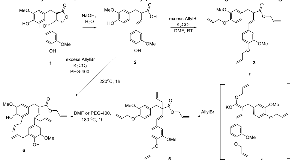
Figure 1. Reaction
