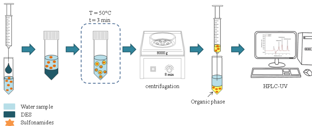
Figure 2. Schematic representation of the pretreatment procedure.
