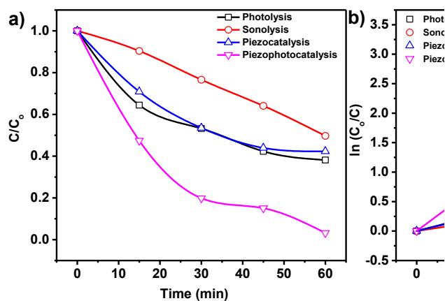
Figure 2. The MB (C=1 mg/l) degradation curves. V = 20 ml, S = 3 cm 2
