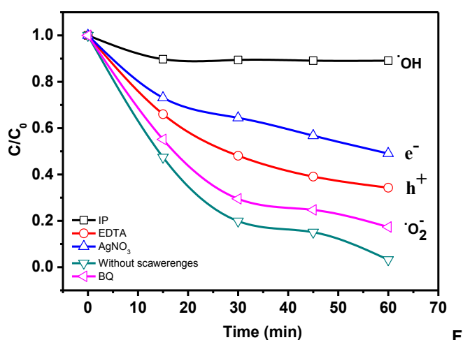
Figure 1. Piezophotocatalytic performance of \alpha\text{-Fe}_2\text{O}_3 containing PVDF nanofibers for degradation of MB under UV-Vis light after adding various scavengers.
