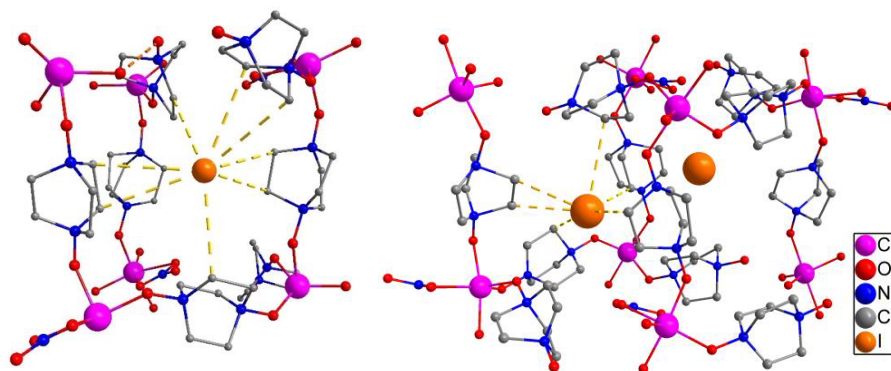
Figure 1. Localization of iodides in cavities in 6 . Dotted lines indicate Co odabco -I distances of less than 4.1 Å.
