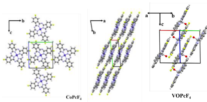
Figure 1. Molecular packing of \text{CoPcF}_4 and \text{VOPcF}_4 .
