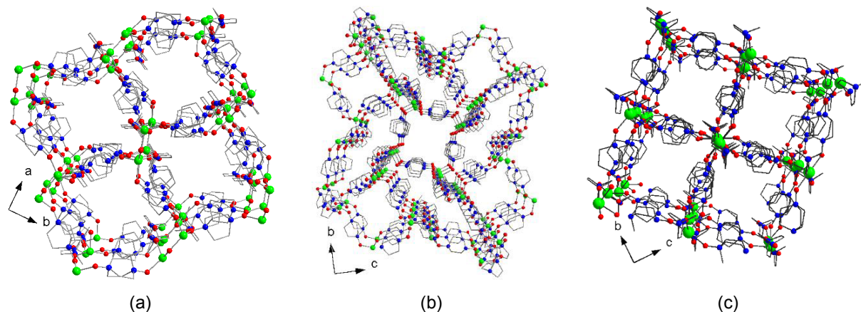
Figure 1. View along the channels in coordination networks: [Zn 2 ( \mu -O)(odabco) 3 ] 2+ (a, pcu topology); [Zn(odabco) 2 ] 2+ (b, bct topology); [Tb(odabco) 3 ] 3+ (c, pcu topology). H atoms are not shown.
