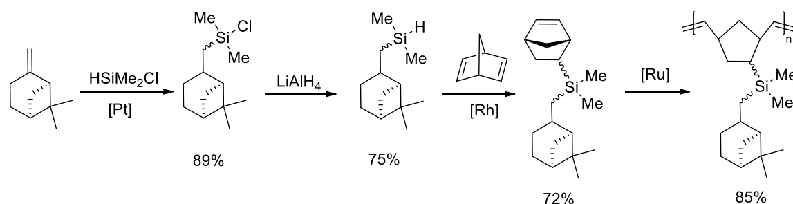
Figure 1. Synthesis of Si-substituted polynorbornene
