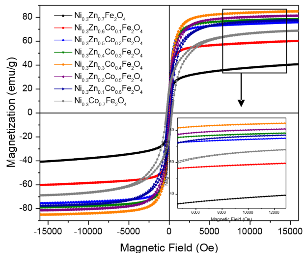
Figure 2. Hysteresis loops of the Ni_{0.3}Zn_{0.7-x}Co_xFe_2O_4 system
