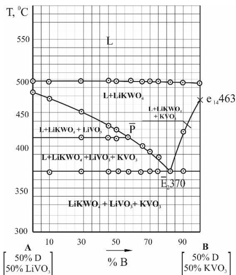
Figure 2. T-x-diagram of a polythermal cut AB
