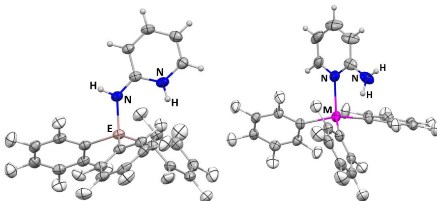
Figure 1. Molecular structures of complexes in crystals. The left one is E(C_6F_5)_3 \cdot C_5H_6N_2 ( E = B, Al ). The right one is M(C_6F_5)_3 \cdot C_5H_6N_2 ( M = Ga, In ).
