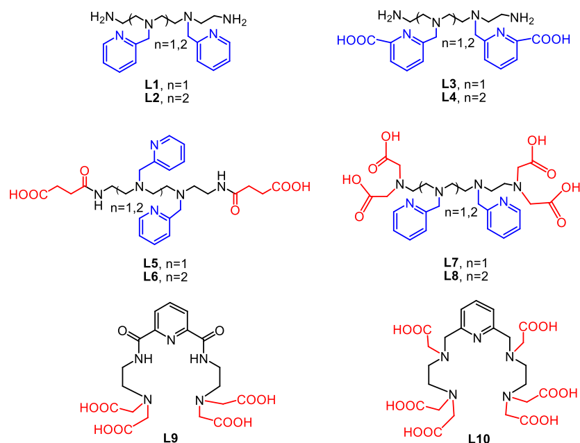
Figure 1. Synthesized ligands.
