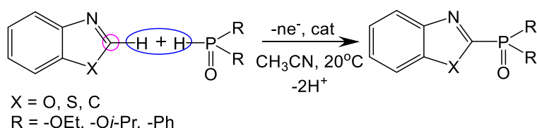
Figure 1. Electrocatalytic oxidative phosphorylation of benzo-1,3-azoles and their analogues
