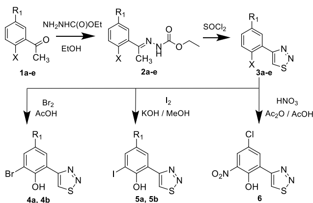
Figure 1. Formation of 1,2,3-thiazoles. 1-3: R_1 = H , X = Br (a); R_1 = MeO , X = Br (b); R_1 = NO_2 , X = Cl (c); R_1 =
