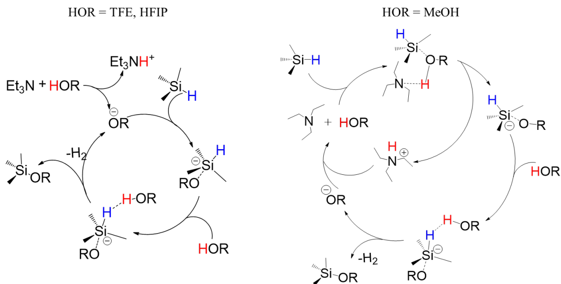
Figure 1. Proposed mechanism of base-catalyzed dehydrocoupling of silanes and alcohols of high ( left ) and low ( right ) acidity.
