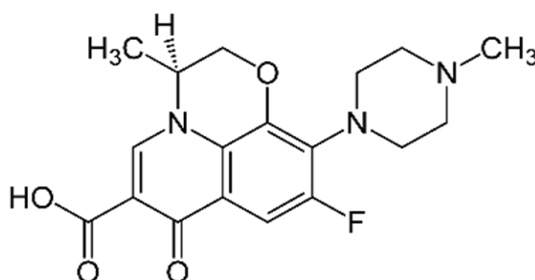
Figure 1. Levofloxacin formula.
