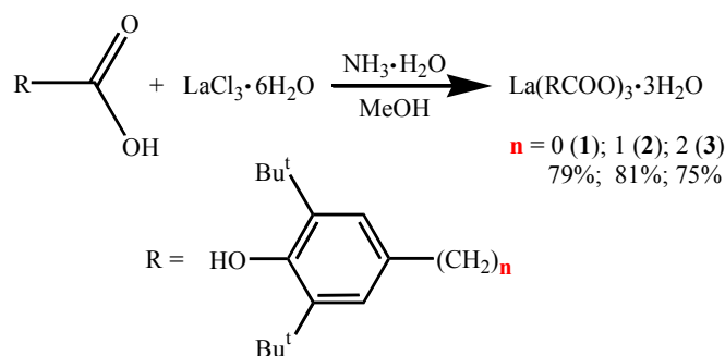
Figure 1. Reaction.
