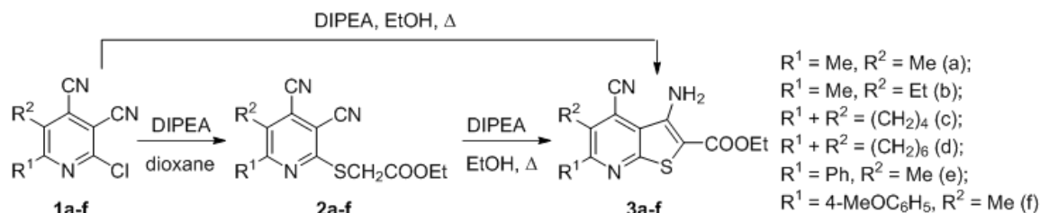
Figure 1. Reaction.
