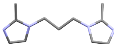
Figure 1. 1,3-bis(2-methyl-imidazolyl)propane (bmip)
