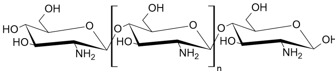
Figure 1. Structure of chitosan.
