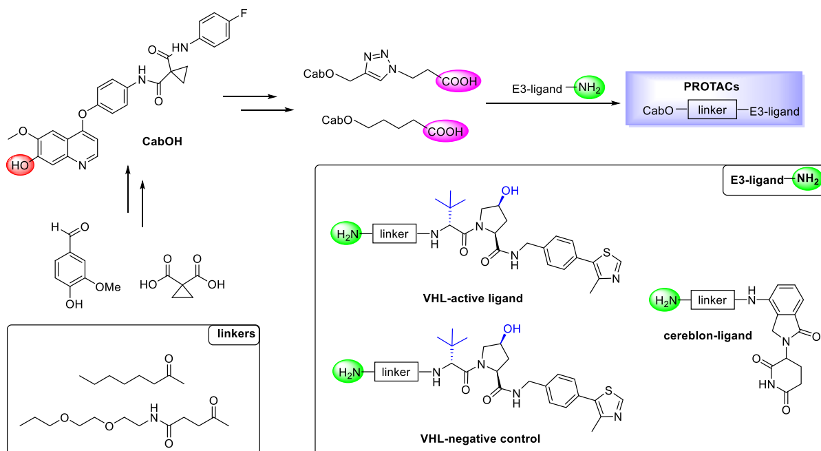
Figure 1. PROTACs synthesis.
