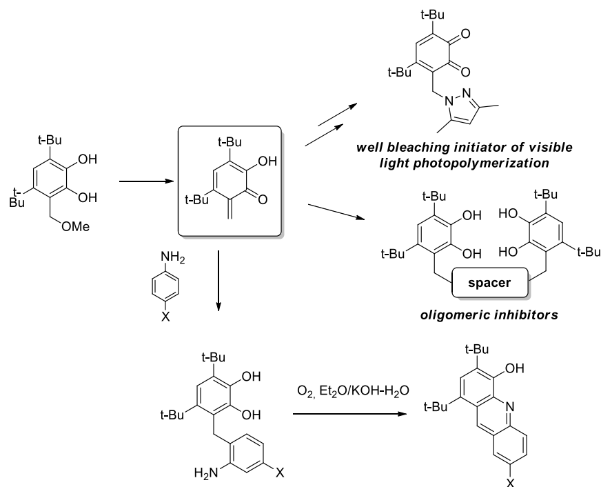
Figure 1. Reaction.
