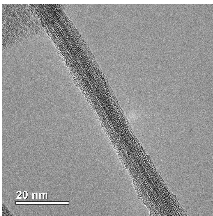
Figure 1. TEM micrograph of E(\text{SbI}_3\text{-Sb}_2\text{S}_3)\text{@SWCNT} nanocomposite.
