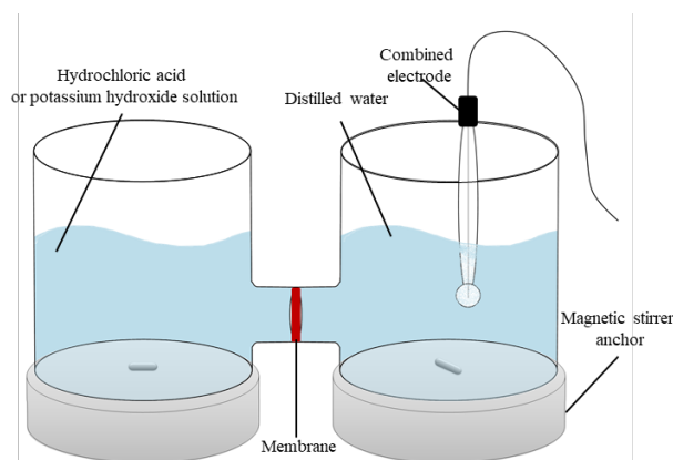
Figure 1. Installation diagram for the experiment.
