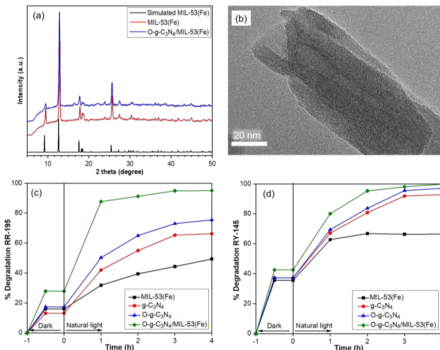
Figure 1. (a) PXRD patterns of simulated MIL-53(Fe), as-synthesised MIL-53(Fe) and O-g-C 3 N 4 /MIL-53(Fe), showing MIL-53(Fe) crystals were successfully formed using the recycled polyethylene terephthalate and the MOF crystallinity was maintained during the facile synthesis of the novel O-g-C 3 N 4 /MIL-53(Fe) composite. (b) TEM image of O-g-C 3 N 4 /MIL-53(Fe) composite disclosing the appearance of multi-walled nanotubes with the onion-like walls. (c) and (d) Photocatalytic degradation of RR 195 and RY 145 using g-C 3 N 4 , O-g-C 3 N 4 , MIL-53(Fe) and O-g-C 3 N 4 /MIL-53(Fe), showing the higher degradation efficiency of the composite material compared to the pristine samples.
