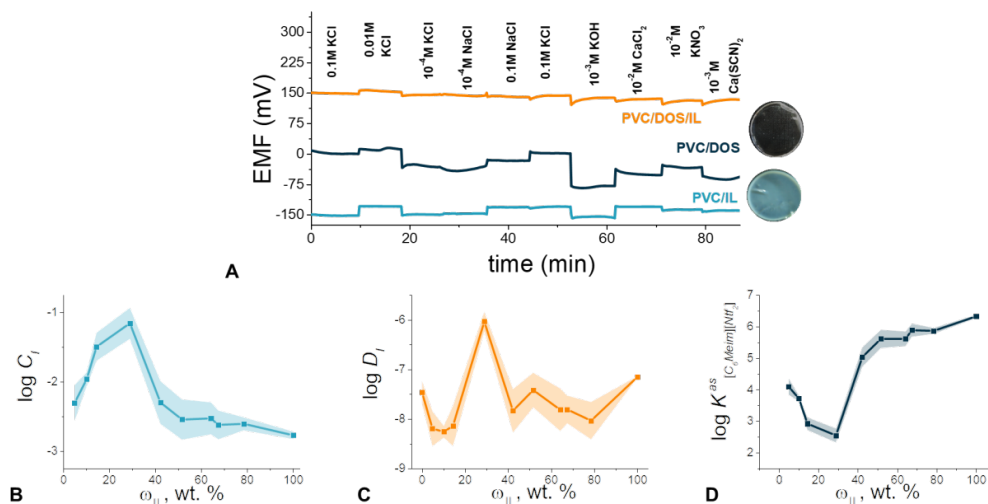
Figure 1. A) EMF of the cell containing the electrodes with membranes plasticized with pure DOS , pure IL , or their mixture. Inset photos: membranes plasticized with pure DOS (top) and pure IL (bottom). B, C, D: dependence of B) concentration of C 6 MeimNTf 2 ions; C) their mean diffusion coefficient; D) association constant, on the C 6 MeimNTf 2 content in the membrane.
