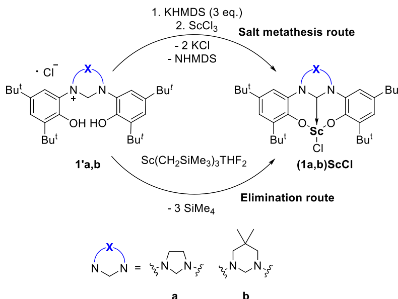
Figure 1. Synthesis of scandium halides
