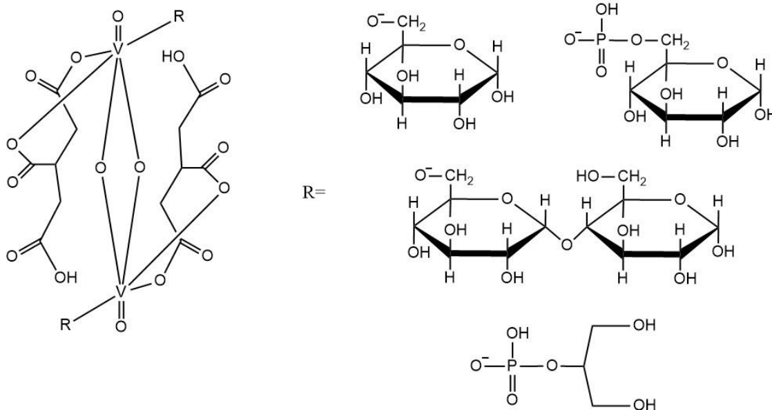
Figure 2. Resulting compounds.
