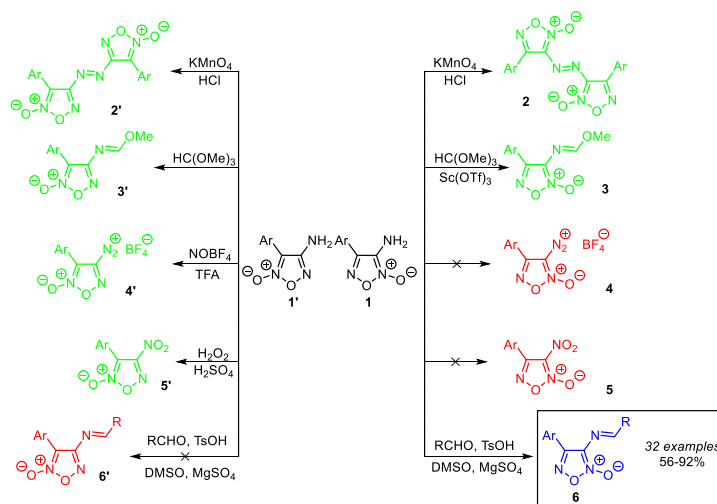
Figure 1. Comparison of reactivity of isomeric aminofuroxans.
