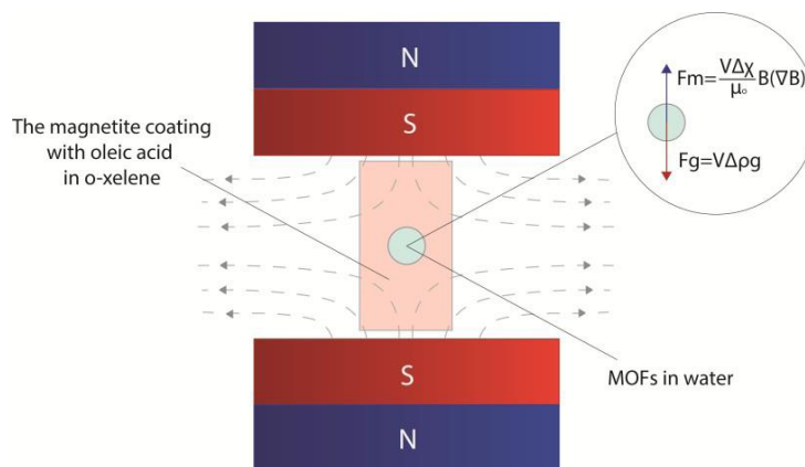
Figure 1. Reaction.
