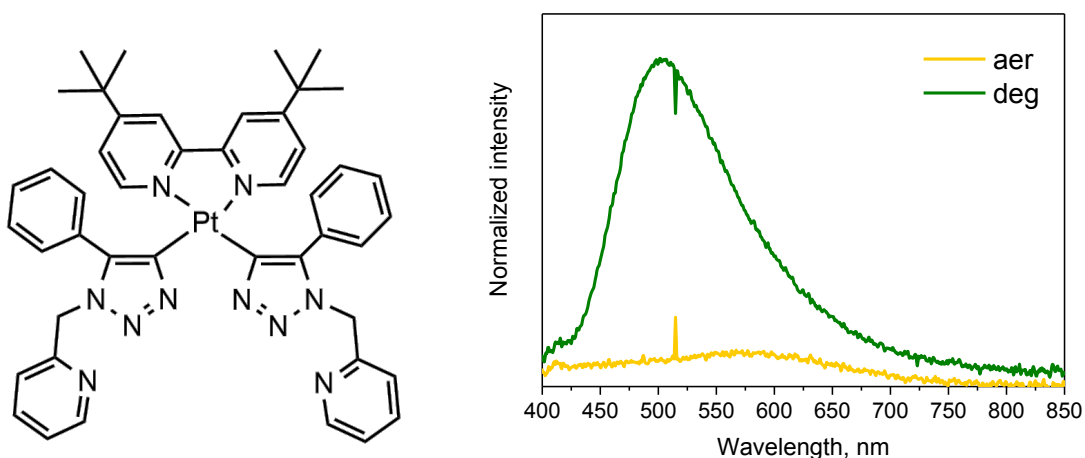
Figure 1. On the left: structure of [Pt(dtbp)(i-click) 2 ]. On the right: Normalized emission spectra for aerated and degassed solutions of [Pt(dtbp)(i-click) 2 ]
