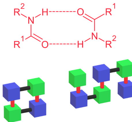
Figure 1. Structural formula of formamide homodimers with various substituents R1, R2 (up) and two alternative types of self- association of the formamide-molecule (down), blue cube is D, green cube is A.
