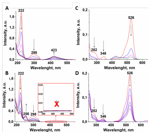
Figure 1. UV-vis spectra for DHN (a,b) and Rh6G (c,d) in presence SURMOF/GO with the pore size of 1.6 nm at aerobic (a,c) and anaerobic (b,d) conditions.
