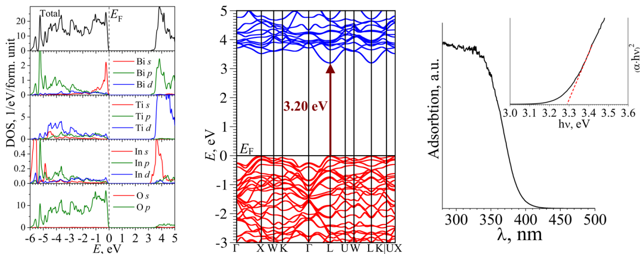
Figure 1. Electronic structure and experimental absorption spectrum of the \text{Bi}_{1.5}\text{In}_{0.5}\text{Ti}_2\text{O}_7 pyrochlore.
